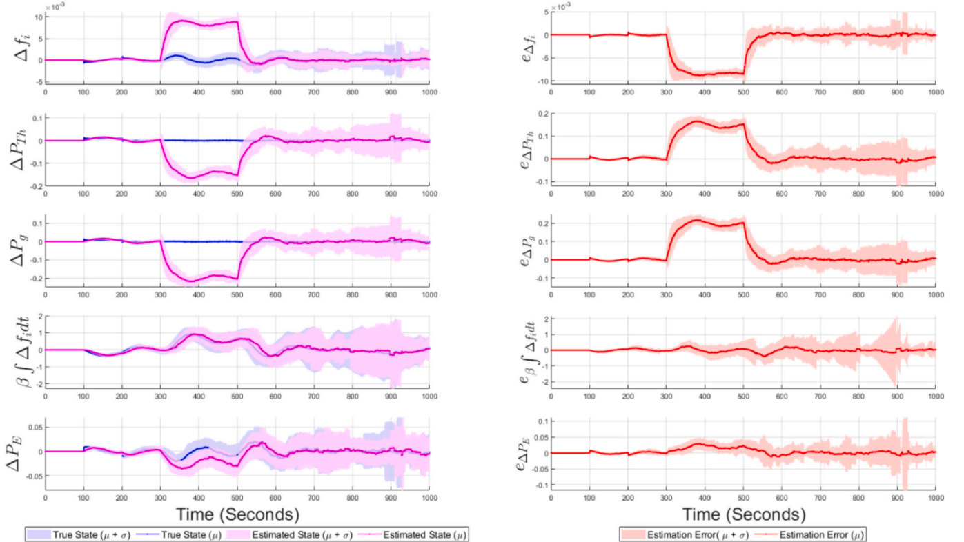
Fig. 10. True/observed states for LFC with decentralized EV configuration under bounded noise and disturbance obtained after 100 Monte Carlo simulations at 99% random packet drop rate.
