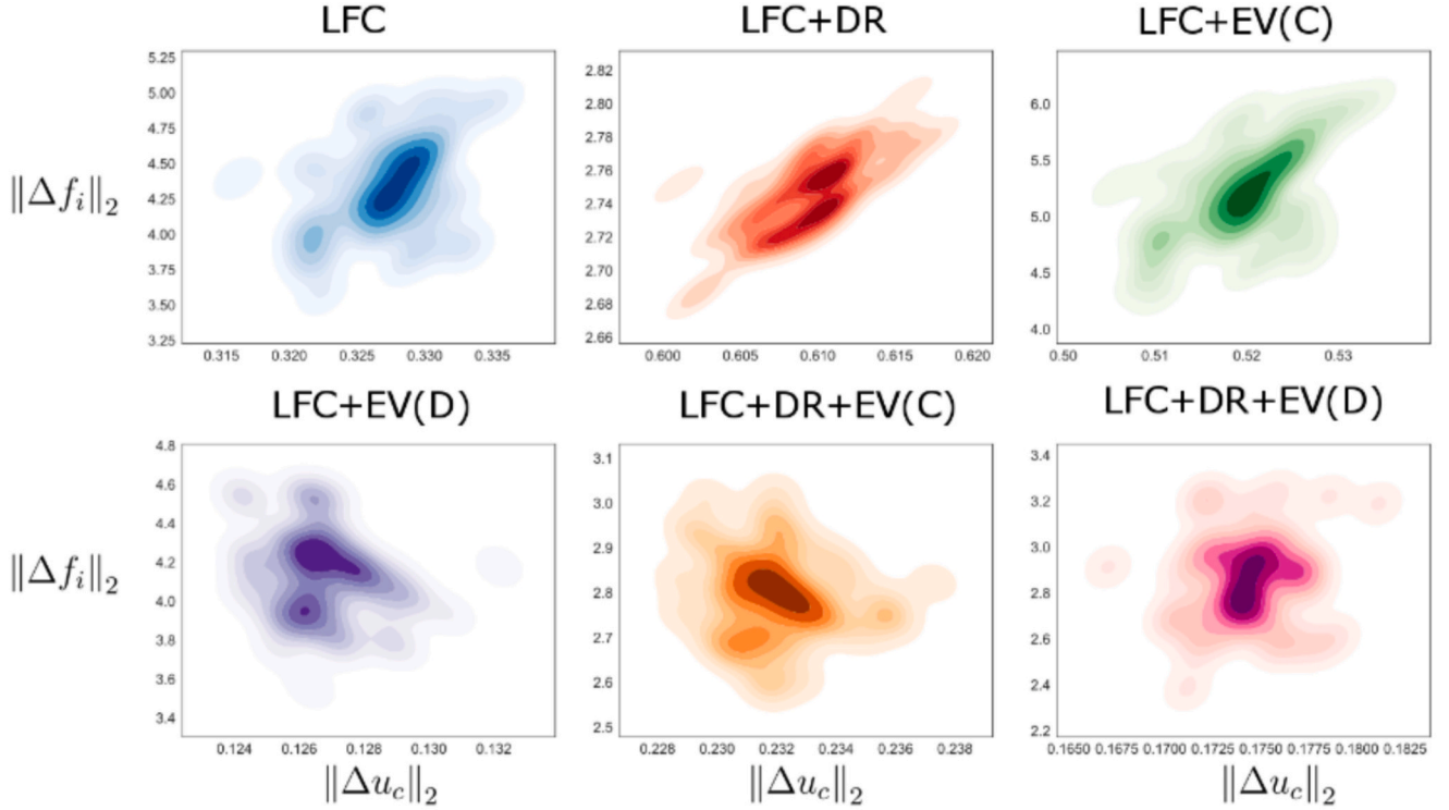
Fig. 29. Bivariate analysis of the L_2 -norm of the frequency fluctuations and governor control input with 500 Monte Carlo simulations.
