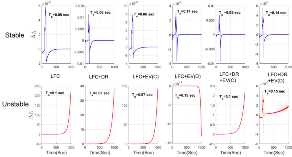
Fig. 4. Stable and unstable system response for different sampling time for different LFC system configurations.
