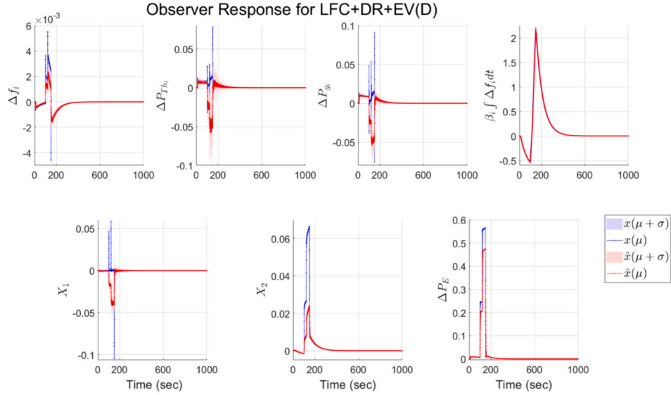
Fig. 18. Observer response for LFC, DR and decentralized EV system configuration with mean and uncertainty calculated over 100 Monte Carlo simulations.
