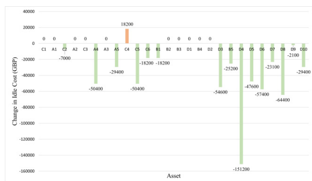
Fig. 7: Change in Idle Cost of ships after optimisation.
