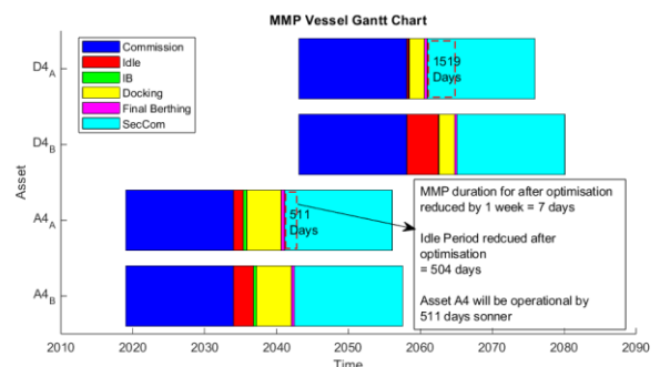
Fig. 6: Shows sample of MMP activities for ships with reduced waiting period after optimisation.
