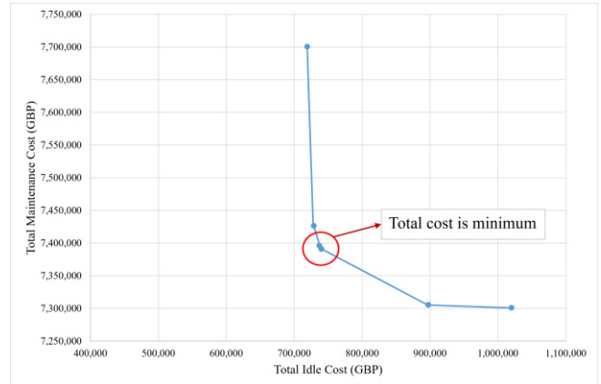
Fig. 4: Plot of Idle Vs Maintenance cost for the optimal docking values obtained from experiments in Table 2.
