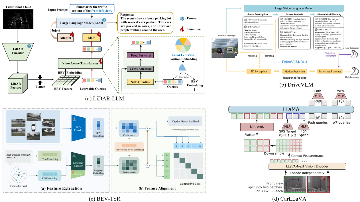
Figure 4. Some representative studies related to the application of LLMs and MLMs in perception.
