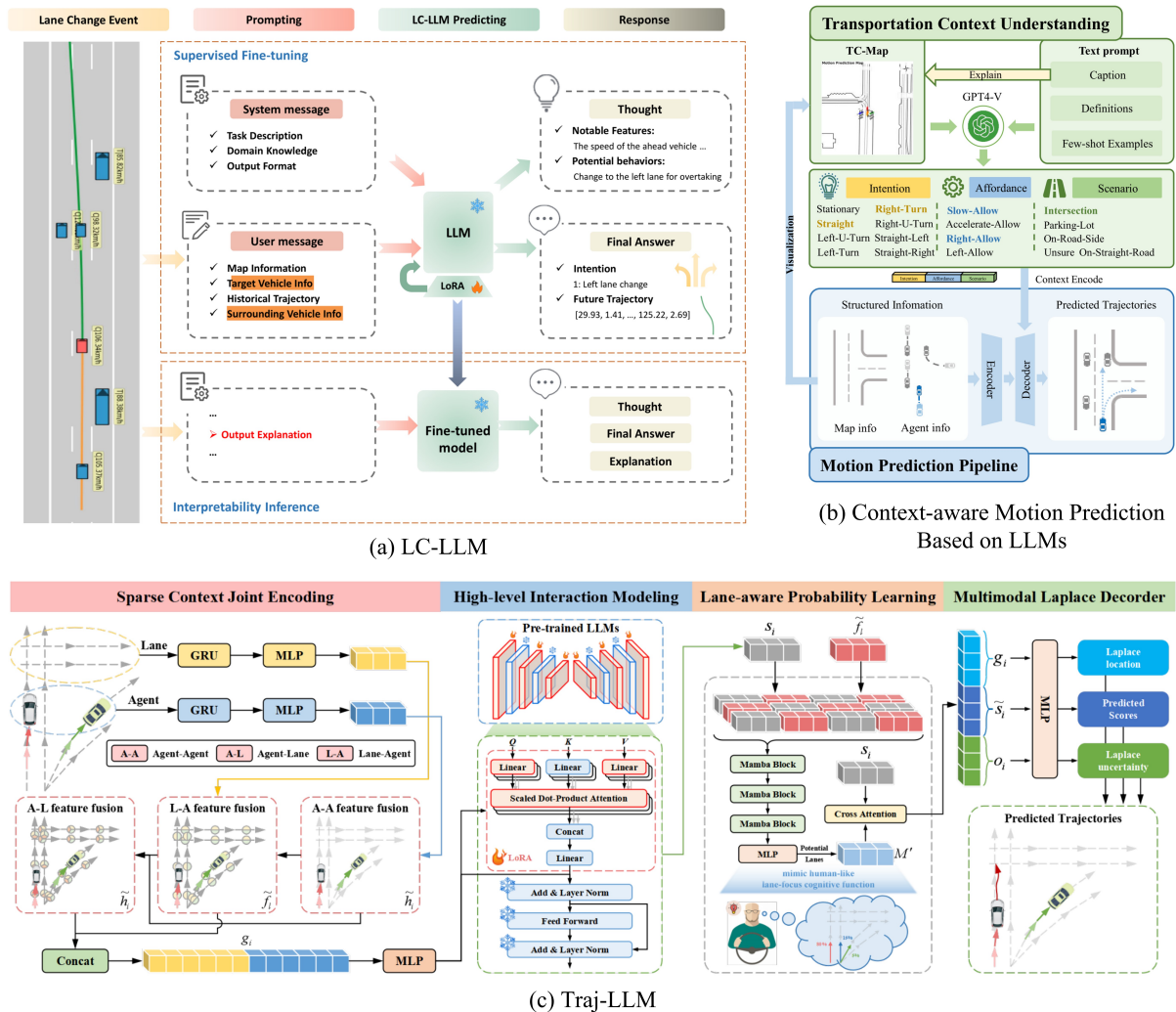
Figure 5. Some representative studies related to the application of LLMs and MLs in prediction.
