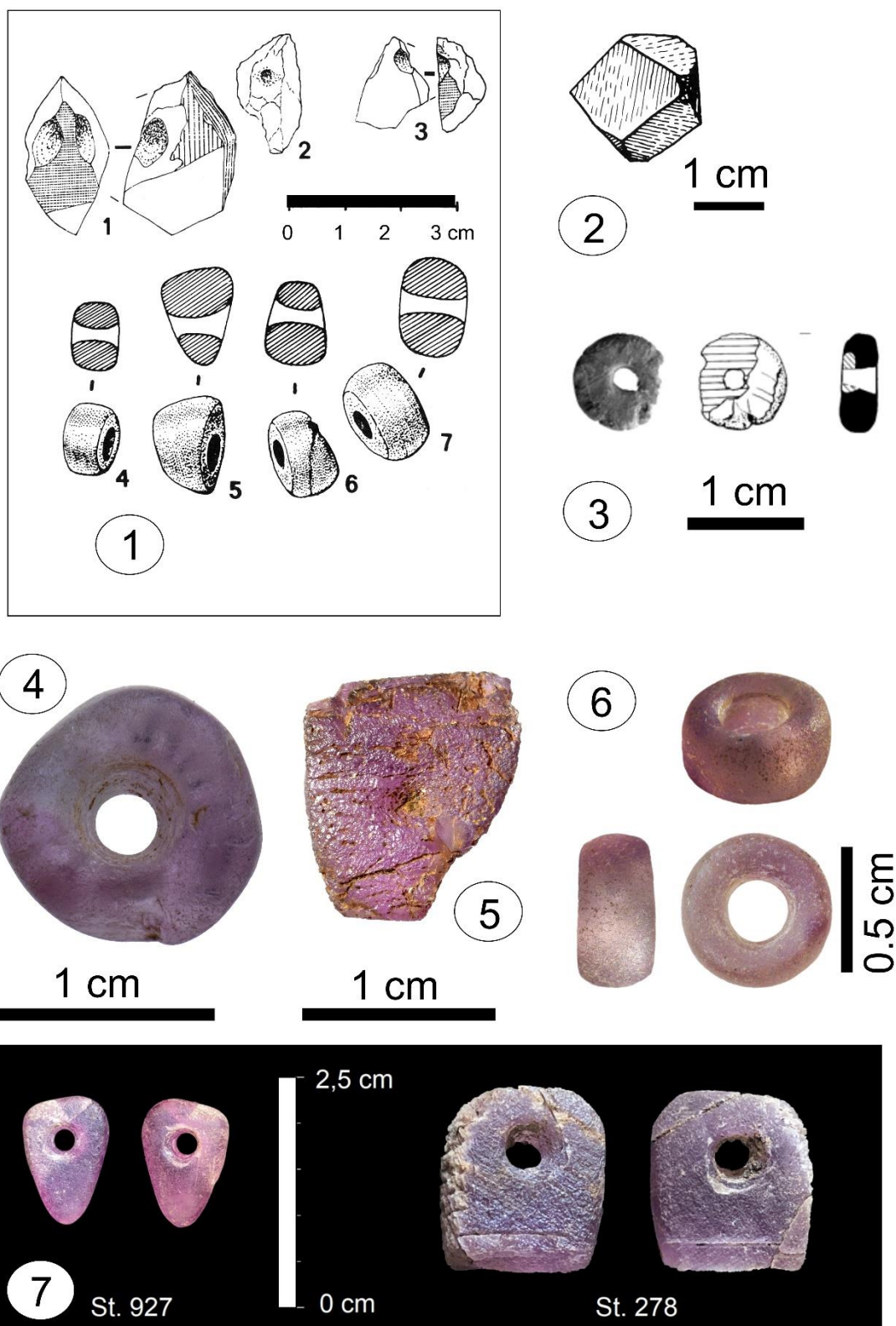
Fig. 2. A sample of pearls and fragments of archaeological fluorite described and analysed in this paper. 1) Thieusies (Vermeersch et al., 1990); 2) Neufvilles (De Heinzelin et al., 1977, p. 97, Fig. 43, n° 9); 3) Spiere (Vanmontfort et al., 2001/2002, p. 55); 4) Namur (D. Bosquet, AWaP); 5) Olloy-sur-Viroin (P. Cattelain, CEDARC-Musée du Malgré-Tout); 6) Mairy (Fourny and Van Assche, 2020), and 7) Passel (N. Cayol, Inrap).
