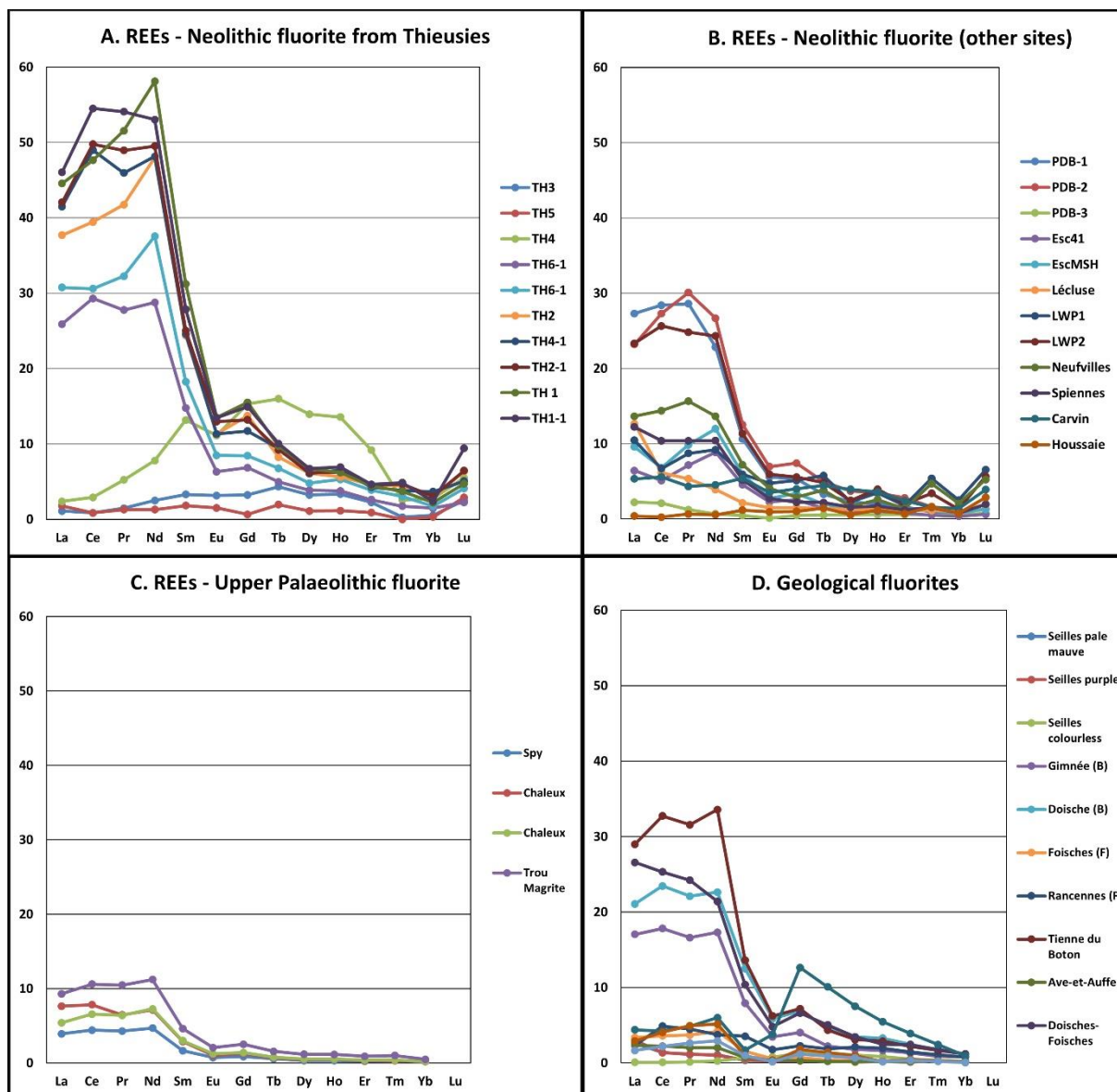
Fig. 6. Chondrite-normalised REE contents in archaeological fluorites. a) Fluorite from Thieusies; b) Fluorites from other Neolithic sites; c) Upper Palaeolithic fluorites; d) Geological fluorites. Values normalised after Sun and MacDonough (1989).
