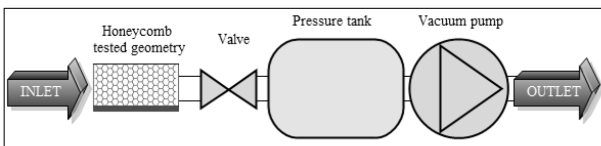
Figure 1. Test rig scheme
