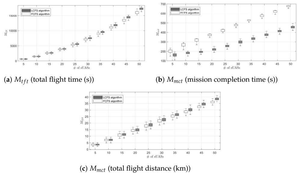
Figure 10. 1-to- \mathcal{M} Case: Standard deviation comparisons between the FCFS algorithm and the LCFS algorithm for M_{ift} , M_{mct} , and M_{ifd} .
