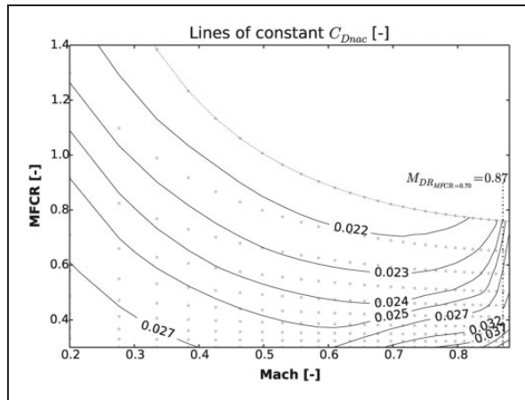
Figure 15. Effect of the MFCR and M_\infty on C_{D_{nac}} for the E1 engine at different Mach numbers.
