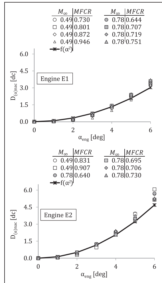
Figure 20. Increase in D_{nac} due to the increase in \alpha_{eng} for two engines at different operating conditions and computed with f(\alpha_{eng}^2) . C_{D_{nac}} [dc] = 10^4 \frac{D_{nac}}{q_\infty S} .
