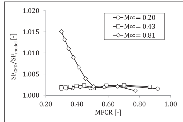
Figure 16. Ratio between the SF computed in CFD studies and estimated by the Reynolds model (equation (17)) for the E2 and E1 engines.
