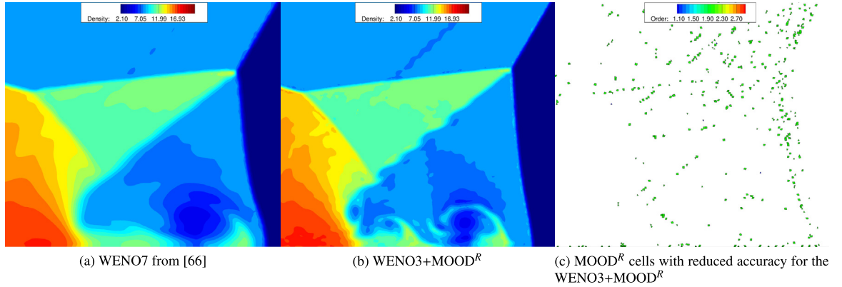
Fig. 9. Zoomed on the wave interaction zone for the double Mach reflection problem, where the key differences can be noticed between the WENO3 with a posteriori MOOD R -limiting, and the results obtained with a WENO 7th-order scheme on a finer mesh as reproduced from [66]. The structures related to the shear waves appear more pronounced in the finer-resolution results with WENO7 as expected, and the figure on the right highlights the locations of the cells for which the MOOD R -limiting approach has reduced their spatial accuracy.
