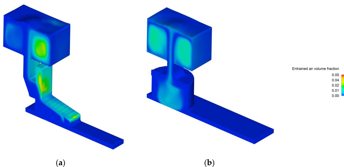
Figure 9. Entrained air volume fraction profiles for the (a) trident gate (TG) and (b) vortex gate (VG) designs.
