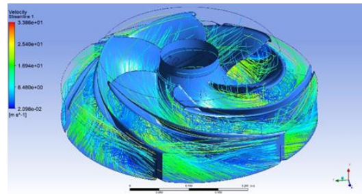
Fig. 5. The value of fluid velocity on impeller
