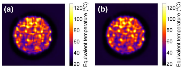
Fig. 8 a A typical thermal image recorded at the output of a coiled 1000 \mu\text{m} bore waveguide transmitting the QCL beam and b the thermal image after up-sampling and interpolation to remove the pixellation
