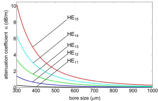
Fig. 3 Variation of the attenuation coefficient \alpha_{lm} with bore diameter for the five lowest order \text{HE}_{lm} modes at 7.8 \mu\text{m} . The high attenuation of higher-order modes for the smaller bore diameters means that HSW can transmit a single mode under certain conditions if the bore diameter is small enough
