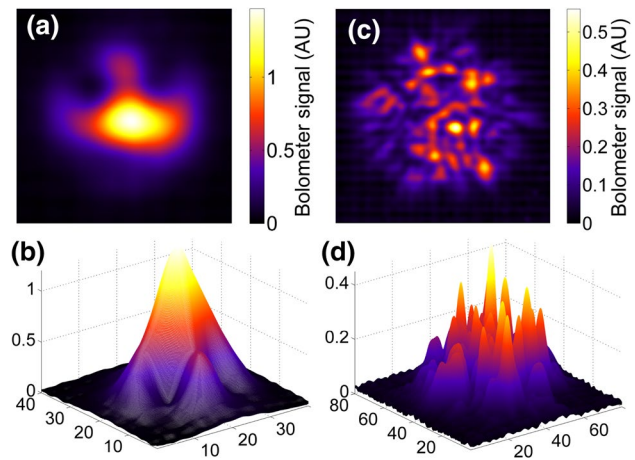
Fig. 16 Intensity distributions detected at the outputs of 5-m coiled lengths of the 300 \mu\text{m} waveguide a and b and the 1000 \mu\text{m} waveguide c and d using a micro-bolometer array beam profiler
