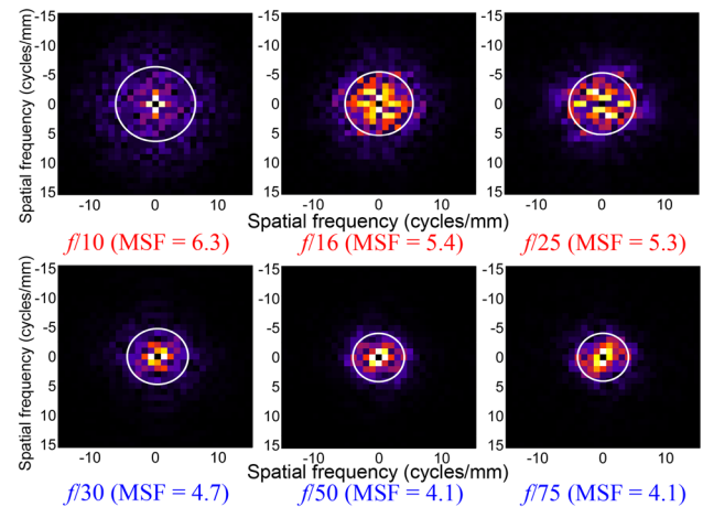
Fig. 13 Fourier transforms of intensity distributions recorded through 1000 \mu\text{m} bore diameter HSW. The rings indicate the mean spatial frequency (MSF) in each image, which is given numerically in brackets below each
