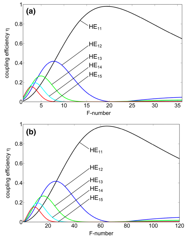
Fig. 4 Coupling efficiency \eta for the five lowest order \text{HE}_{lm} modes plotted against increasing f-number for a a 300 \mu\text{m} bore diameter waveguide and b 1000 \mu\text{m} bore diameter waveguide
