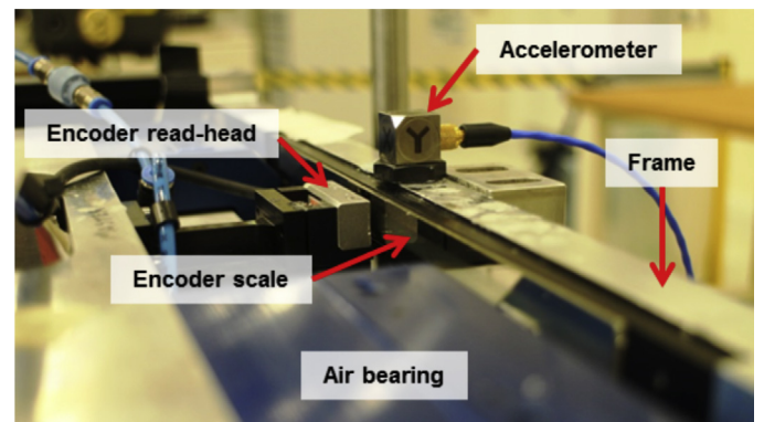
Fig. 7. Accelerometer fixed as close as possible to the encoder scale.
