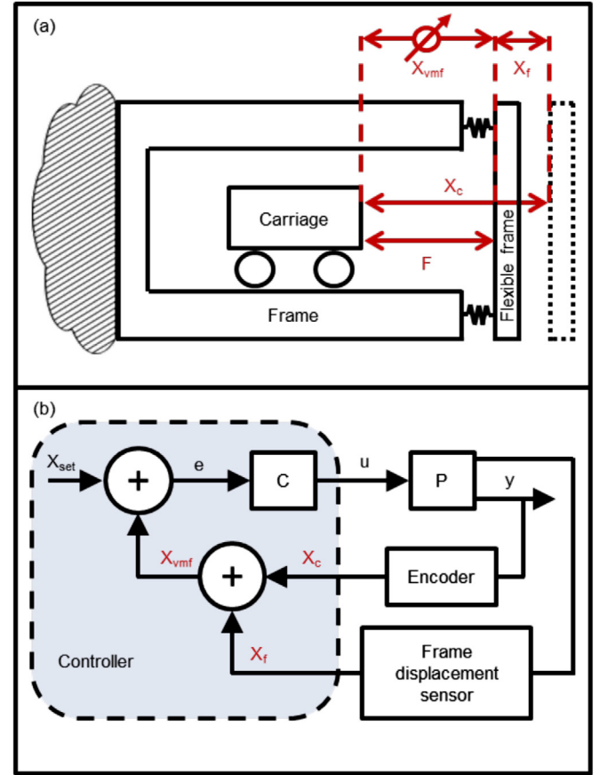
Fig. 1. The Virtual Metrology Frame (VMF) concept.
