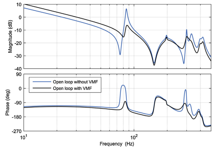
Fig. 12. Open loop Bode plot with and without the Virtual Metrology Frame (VMF) concept.
