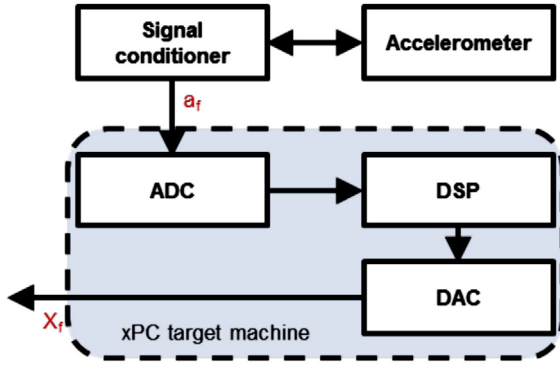
Fig. 8. Frame displacement sensor block diagram.
