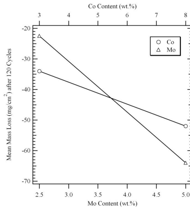
Figure 2 Output from the DoE showing the detrimental effects of increasing Co and Mo contents on the 1100°C cyclic oxidation resistance of the bare LDSX alloys.
