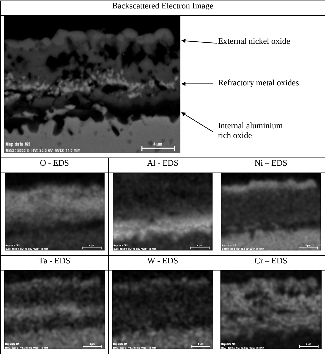
Figure 3 Backscattered electron image and EDS compositional maps of typical bare LDSX-1 1100°C cyclic oxidation microstructure after 200hs
