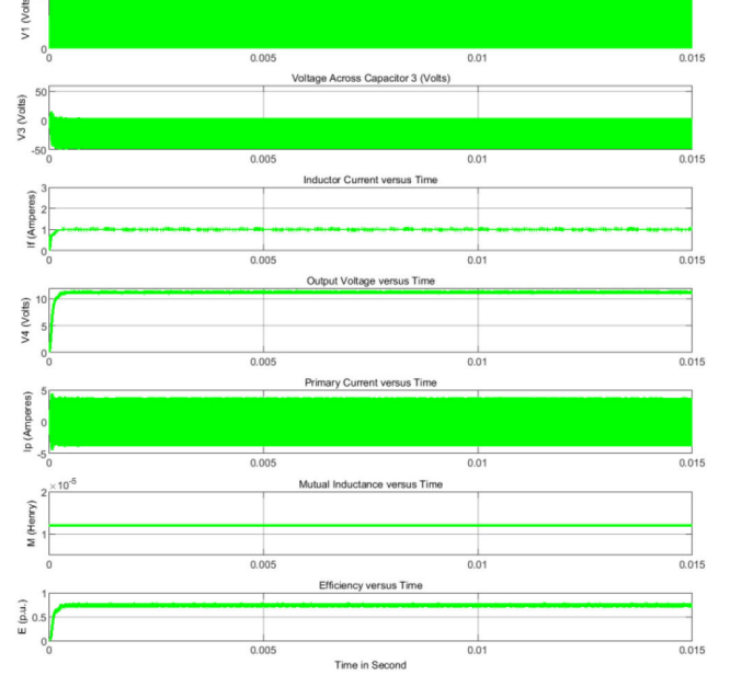
Fig. 10 Results for the converter when f = 217.243 kHz, R_L = 10 \Omega , D_1 = 0.444 , D_2 = 0.501 , delay angle of switch two = 230.1^\circ , k = 0.55 , separation = 3 mm
