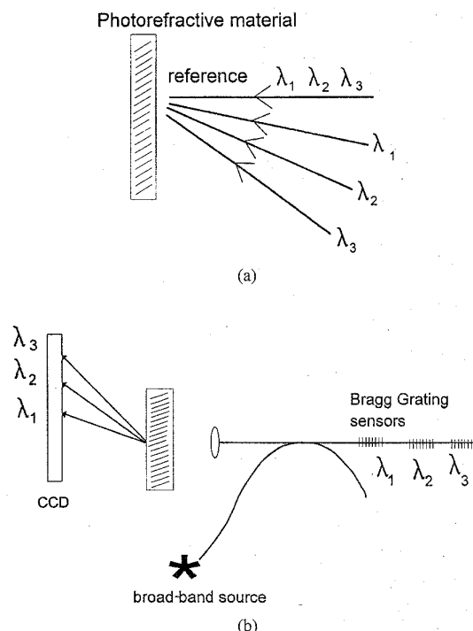
Fig. 1. Concept of the proposed Bragg grating sensor demultiplexing scheme. (a) Recording the holographic filter bank using wavelength-angular multiplexing. (b) Illuminating the filter bank with the reflected Bragg grating signals angularly separates the signals. The diffracted power depends upon the Bragg wavelength shift.
