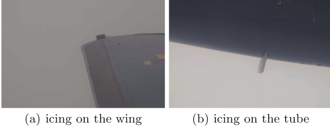
Fig. 2. Natural icing accretion during flight test.
