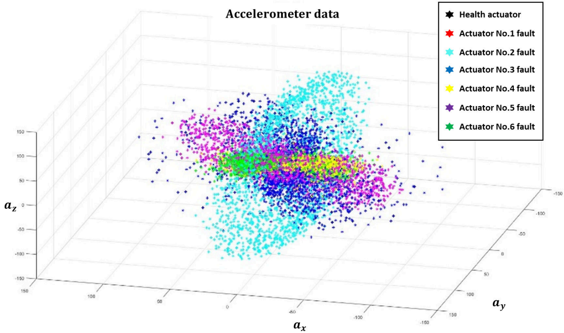
Fig. 9 Scatter plot of accelerometer data in a 3-D feature space
