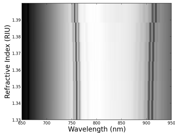
Fig. 9. Evolution of the transmission spectrum of the device in response to a change in the surrounding RI.
