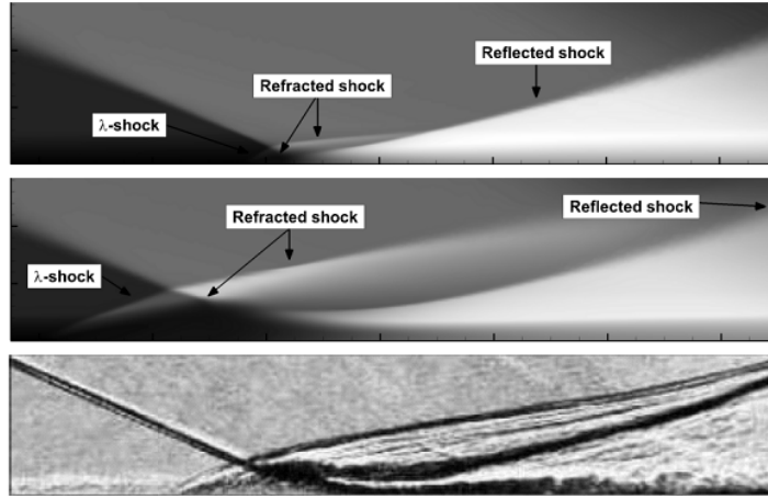
Figure 15. Density contours in comparison with the Schlieren visualization for \beta = 14^\circ (from top to bottom: SU2 SA model, SU2 k-\omega SST model and the experiment of Schuelein et al. [27])
