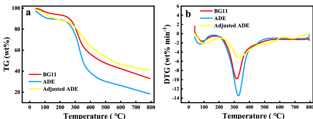
Fig. 2. Thermogravimetry and derivative thermogravimetry analysis of pyrolysis process.
