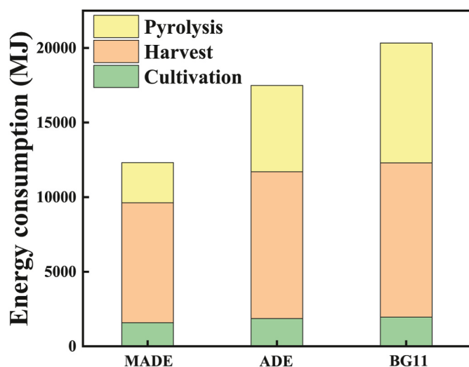
Fig. 4. Energy consumption distribution.
