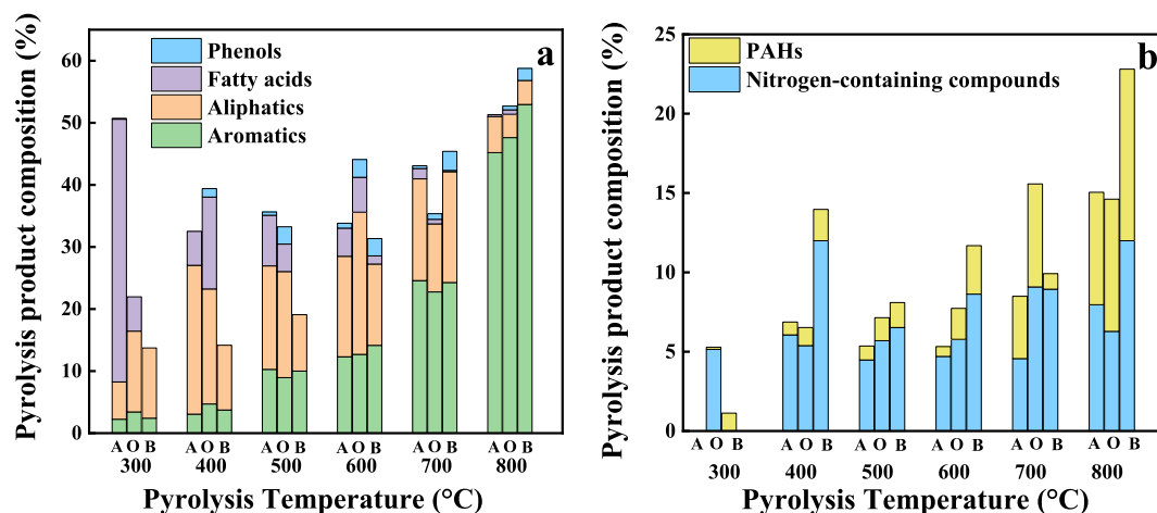
Fig. 3. Pyrolysis products of microalgal biomass cultivated from BG11 medium, anaerobic digestion effluents, and adjusted anaerobic digestion effluents, a) valuable compounds, and b) toxic compounds (A: adjusted AD effluents; O: original AD effluents; B: BG11).
