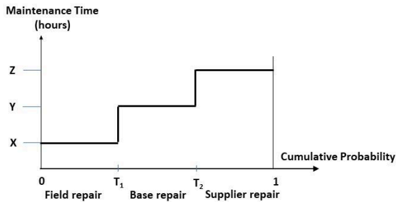
Fig 3. Maintenance time distribution function assumed in modelling.
