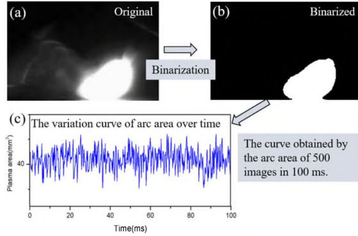
Figure 2. The binarization process of arc images.
