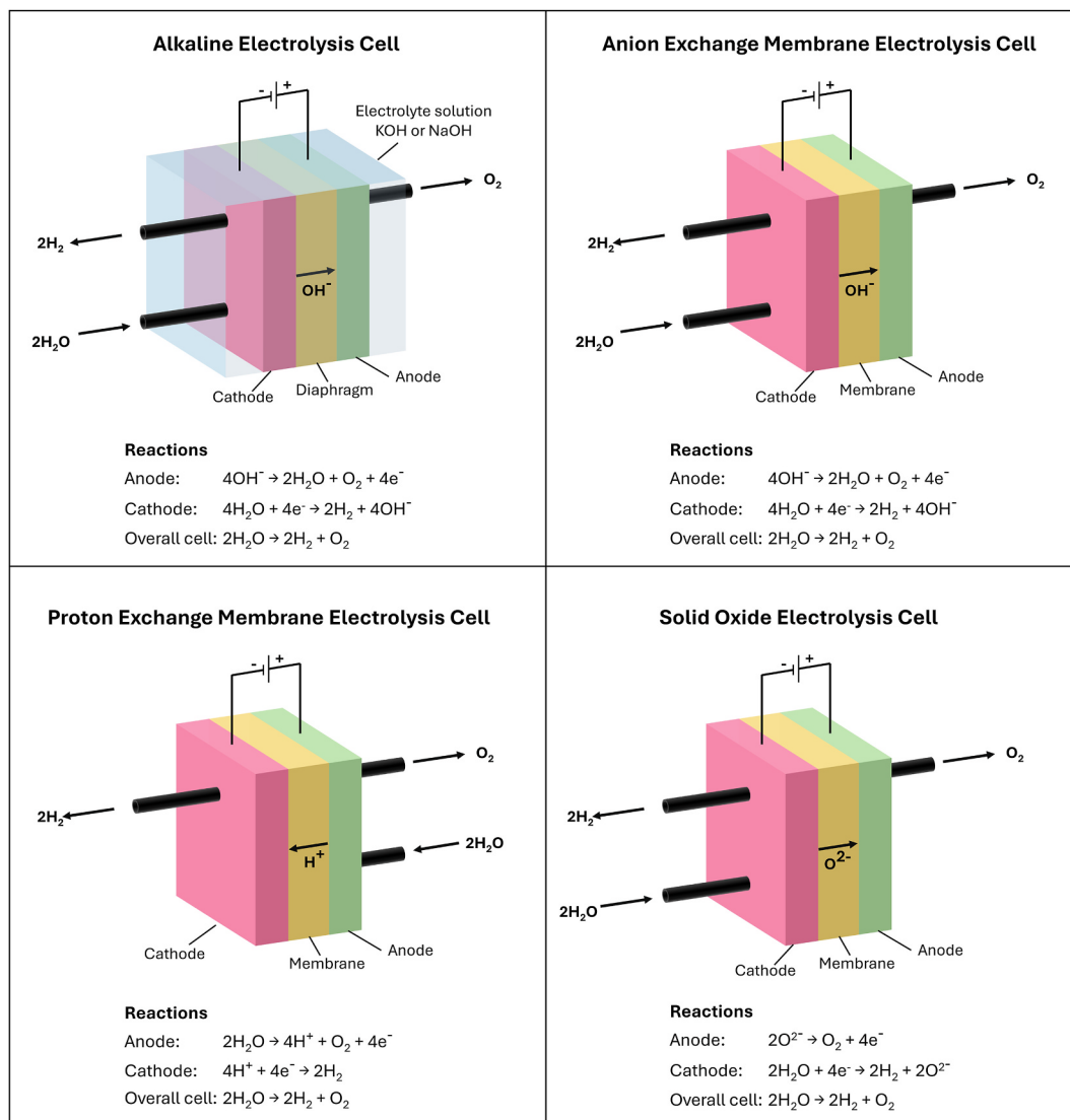
Fig. 3. Schematic of electrolyser technologies.
