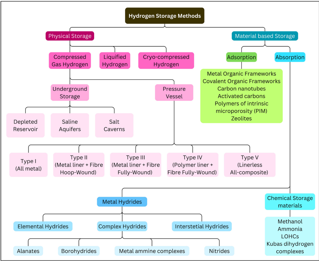
Fig. 6. Hydrogen storage methods.
