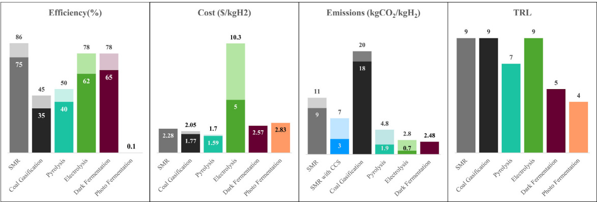
Fig. 5. Comparison of hydrogen production methods.
