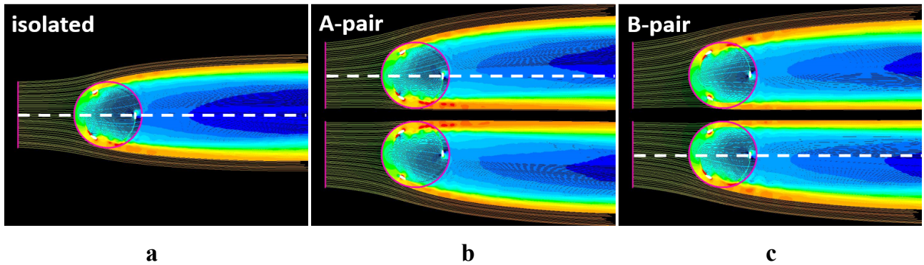
FIGURE 4: Streamlines coloured with velocity magnitude [1÷10.5 m/s] for the isolated turbine (a), A-pair (b) and B-pair (c); to facilitate the comparison, only the streamlines starting from grid cells intercepted by the magenta lines (the same for all the pictures) are shown; white dashed lines indicate the anticlockwise turbines.
