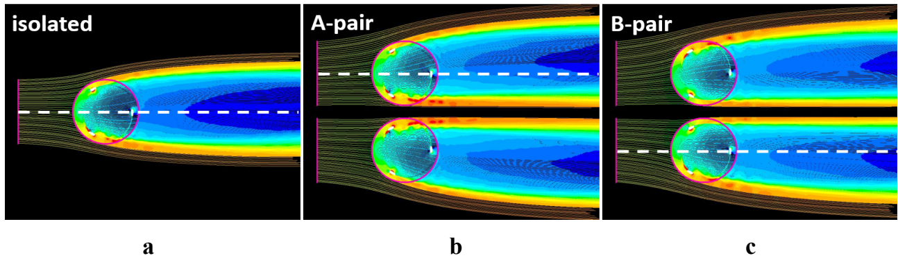
FIGURE 4: Streamlines coloured with velocity magnitude [1 \div 10.5 \text{ m/s}] for the isolated turbine (a), A-pair (b) and B-pair (c); to facilitate the comparison, only the streamlines starting from grid cells intercepted by the magenta lines (the same for all the pictures) are shown; white dashed lines indicate the anticlockwise turbines.
