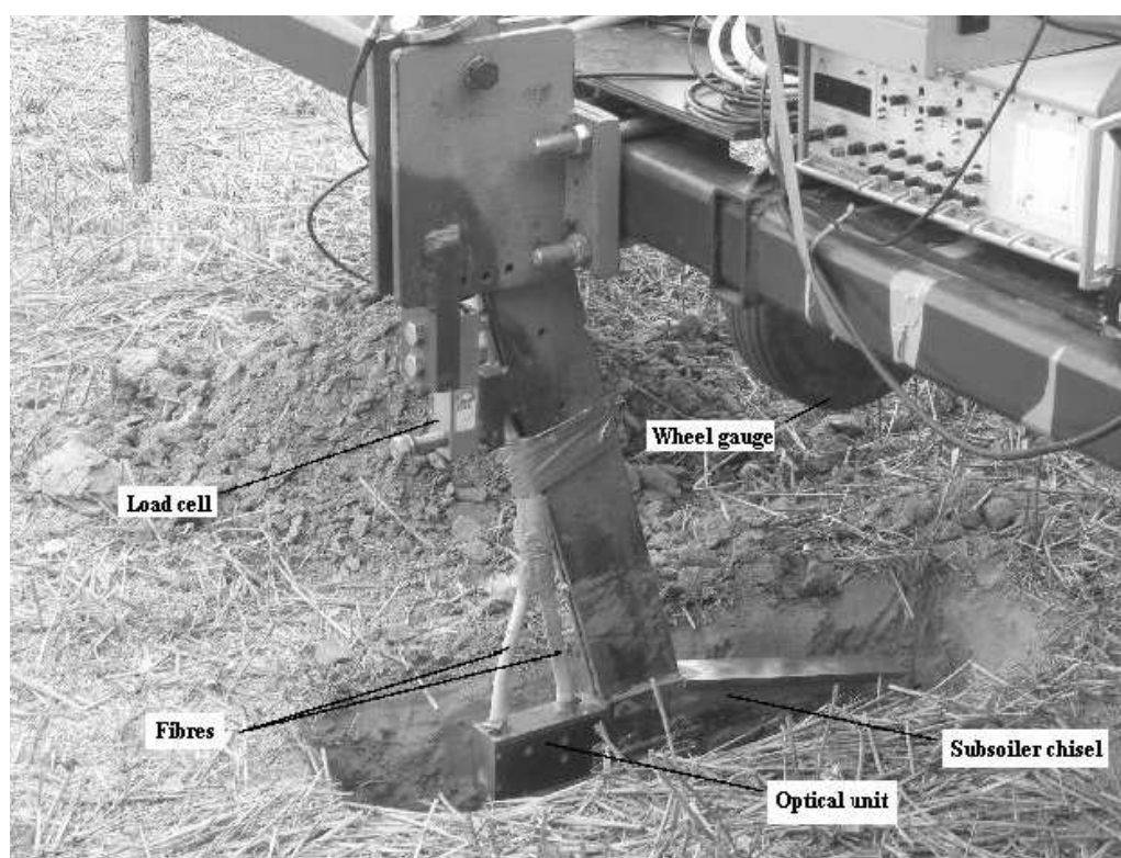
Fig. 1. On-line measurement set up of bulk density (BD) ready for on-line field measurement (after Mouazen et al., 2005)
