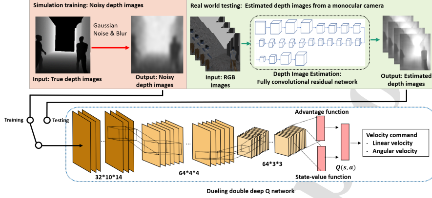
Figure 3: The proposed reinforcement learning framework. In the training phase, noisy depth images are used as an input of D3QN. In the testing phase, the estimated depth images through depth estimation algorithm are used as an input of D3QN. Best view in color.
