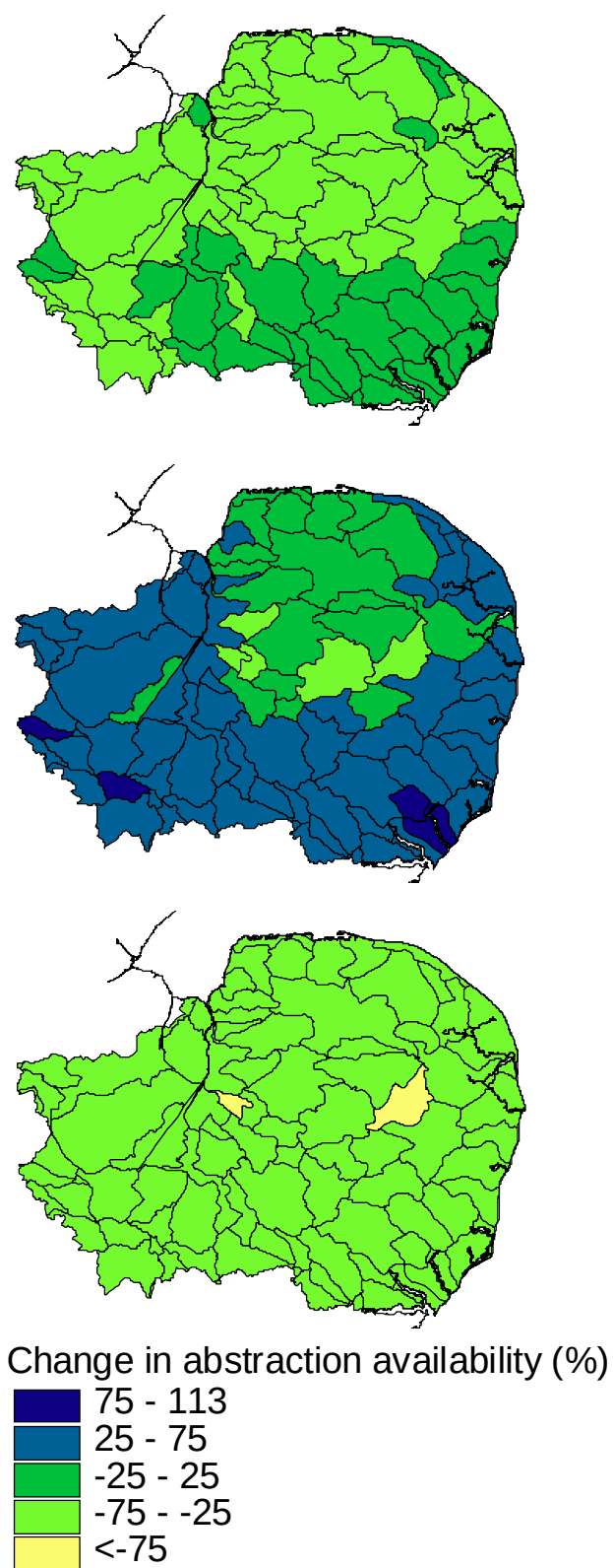
Figure 6: Change in abstraction availability in (upper) Baseline, (middle) Global Markets and (lower) Regional Stewardship futures under 2050s High climate (relative to baseline) for the sub-catchments in East Anglia
