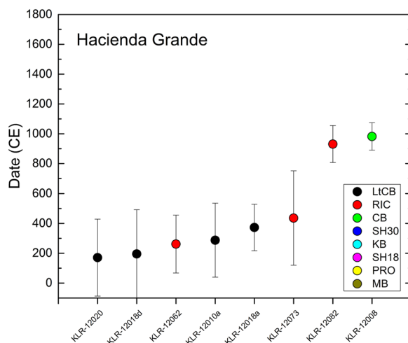
Fig. 8 TL-dates of the Hacienda Grande style. Error bars are 2 standard deviations
