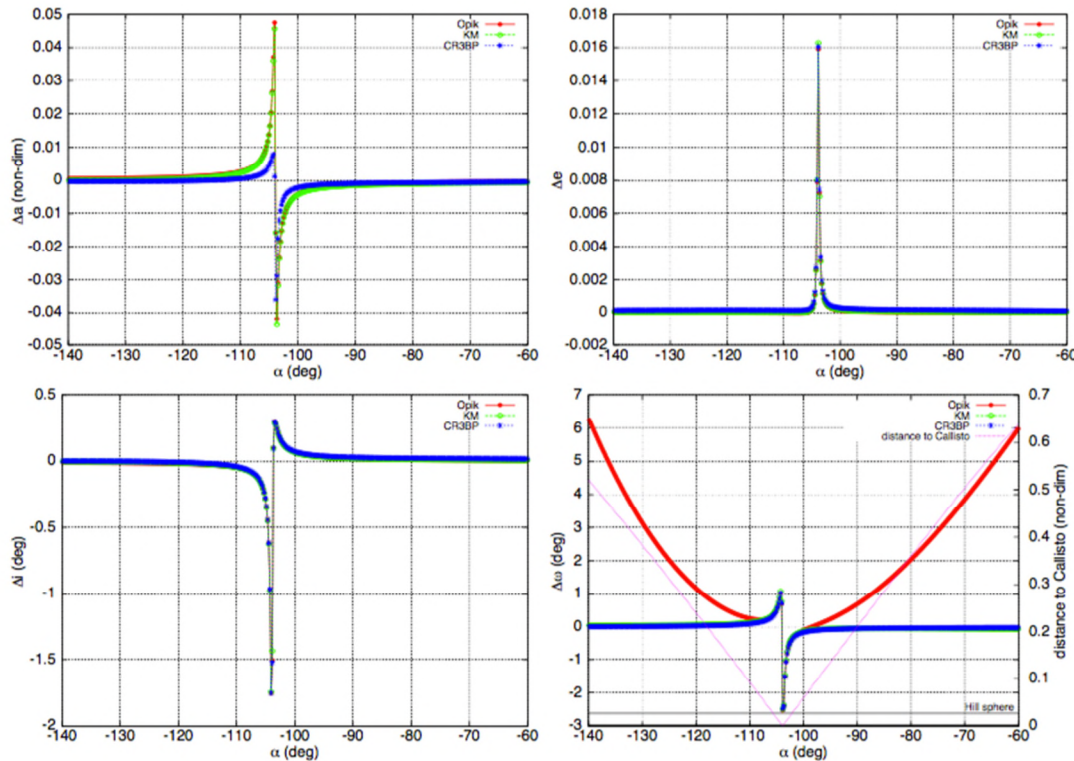
Figure 9. Change in (a, e, i, \omega) induced by Callisto according to the CR3BP, the Keplerian map and Öpik's theory, according to different relative configurations between the spacecraft and the moon, for an initial condition such that T \approx 1.68 and MOID \approx 0.0027 in non-dimensional units.
