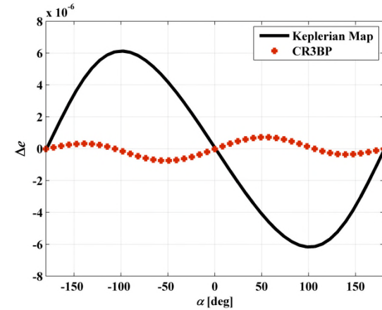
Figure 3. Kick maps for an XMM-like orbit.
