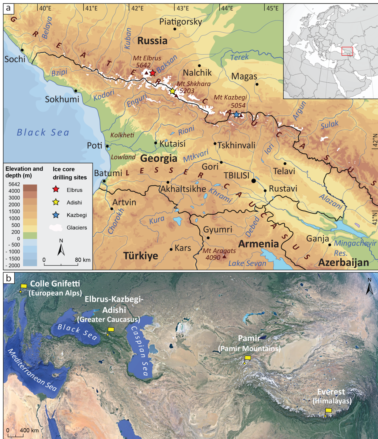
Figure 1. (a)—Location map of Georgia relative to the Caucasus Region and the location of the ice core drilling sites. A physical map of the Caucasus ecoregion was used and modified for the background [31]. The insert map in the upper right shows the location of Georgia relative to Eurasia. (b)—Midlatitude global ice-core locations. (© Google Earth).
