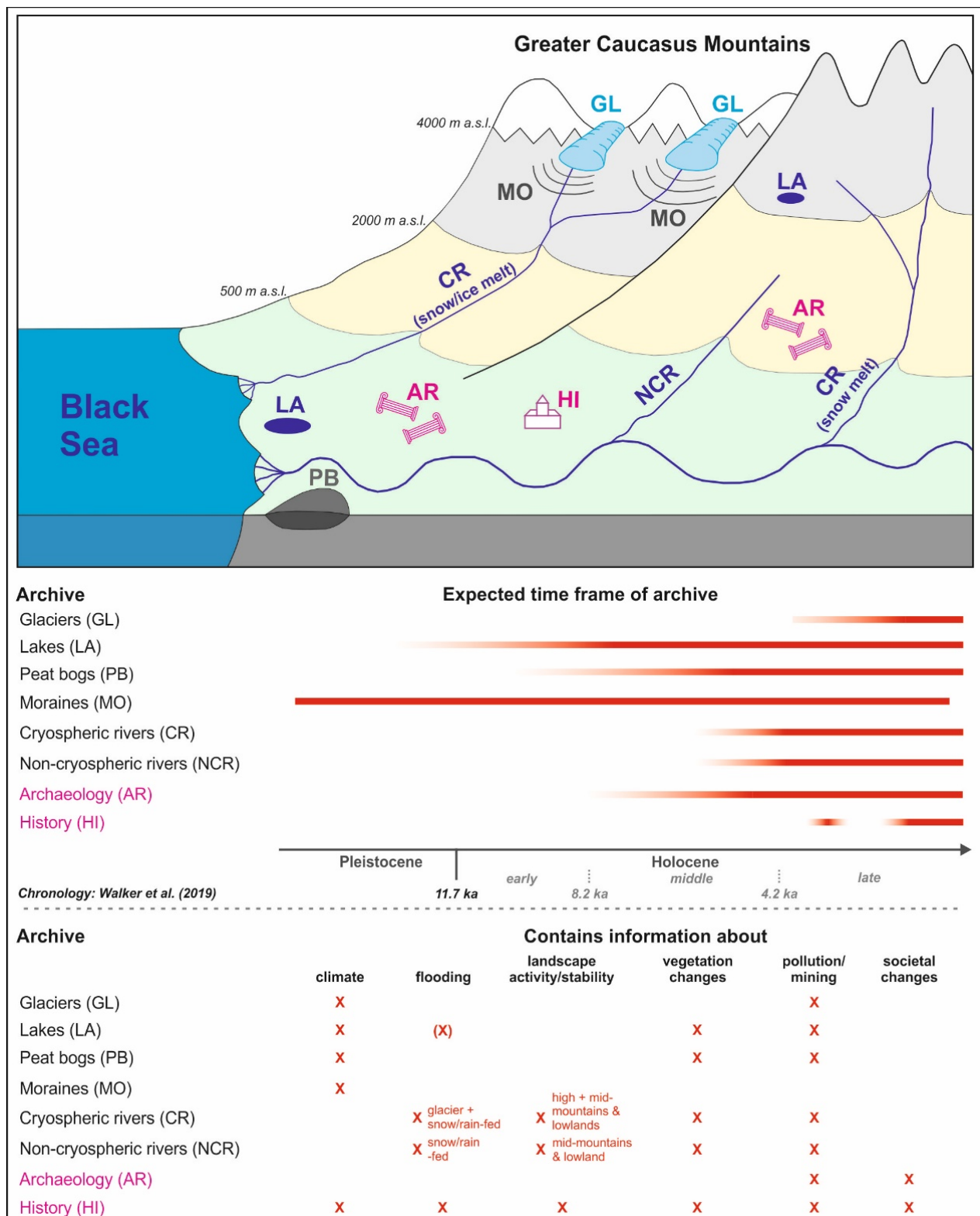
Figure 13. Composite graphic of a transect from the Georgian Greater Caucasus to the Black Sea coast, showing images of the different records at their locations along the transect.
