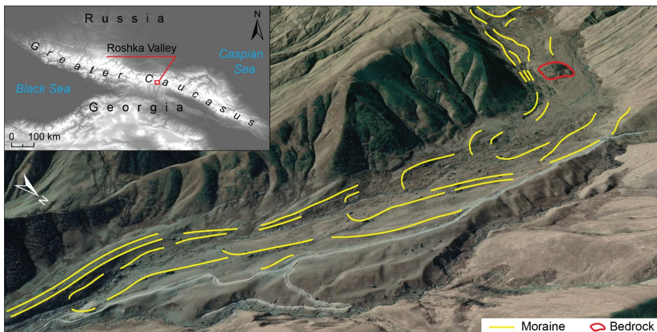
Figure 4. Moraines from the Roshka River valley. Future moraine sampling site. Google Earth image was used as a background. (© Google Earth).
