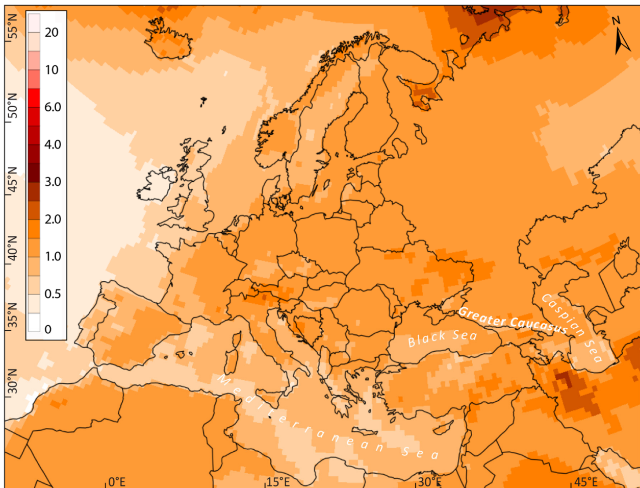
Figure 3. Temperature anomaly plot of observed surface temperature increase in western Eurasia between 2000 and 2023, which has had a very negative impact on many glaciers in the region. The ECMWF European Reanalysis V5 (ERA5) [0.25^\circ \times 0.25^\circ] 2-m surface temperature data files were re-gridded and generated to 0.5^\circ \times 0.5^\circ using bilinear interpolation function. Climate Reanalyzer 2024. [Monthly Reanalysis Maps]. Climate Change Institute, University of Maine. Retrieved [17 January 2024], from https://climatoreanalyzer.org/ .
