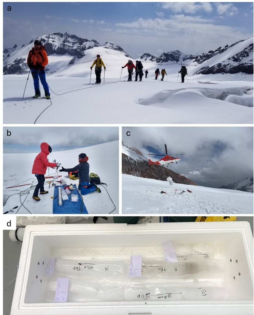
Figure 2. Mount Kazbegi 2021 ice-core pilot project. (a)—ascending to the camping site (4100 m a.s.l.), (b)—Ice sampling site 4300 m a.s.l., (c)—Transportation of the ice samples. (d)—transported ice samples in the laboratory at the Climate Change Institute, University of Maine.
