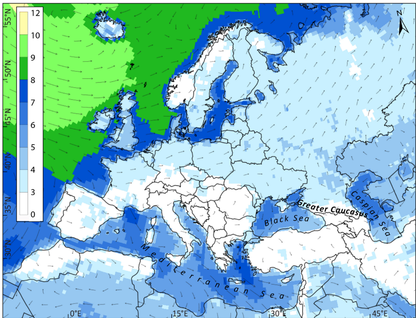
Figure 6. Plot visualising predominant wind directions and wind speed (m/s) in western Eurasia between 2000 and 2023, governing air-mass movement. The ECMWF European Reanalysis V5 (ERA5) [0.5^\circ \times 0.5^\circ] annual data. Climate Reanalyzer™, Climate Change Institute, University of Maine.
