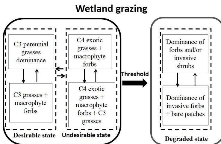
Figure 1. State and transition model for wetland grazing areas using plant functional groups.
