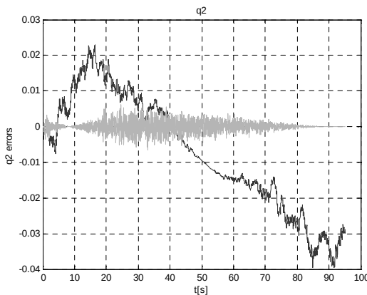
Figure 10. q_2 element errors
