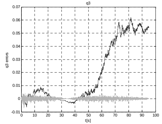
Figure 11. q_3 element errors
