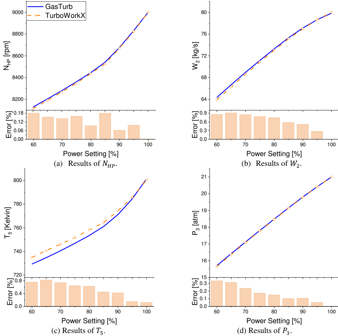
Fig. 7 Model validation at off-design points.
