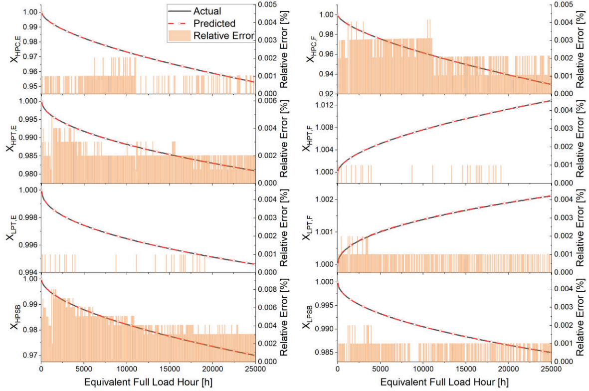
Fig. 12 Actual and predicted degradation factors with fault propagation with EFLH.
