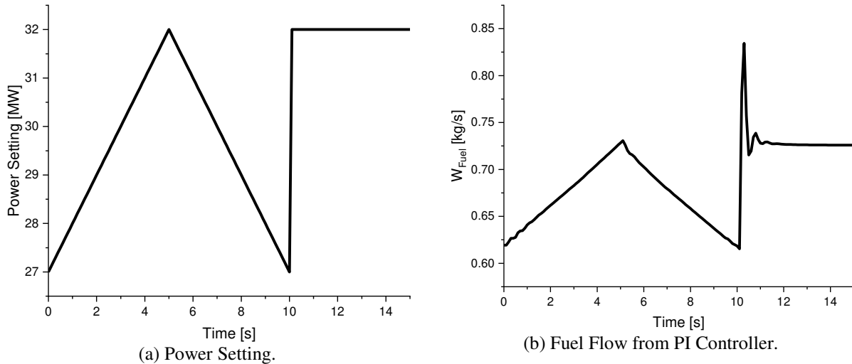
Fig. 13 Power Setting and fuel flow during transient 15 s manoeuvre.
