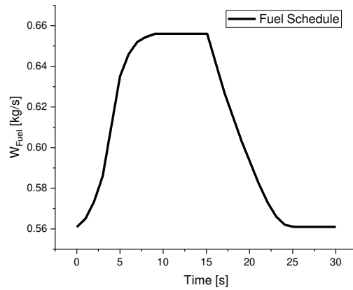
Fig. 8 Fuel schedule for model validation.
