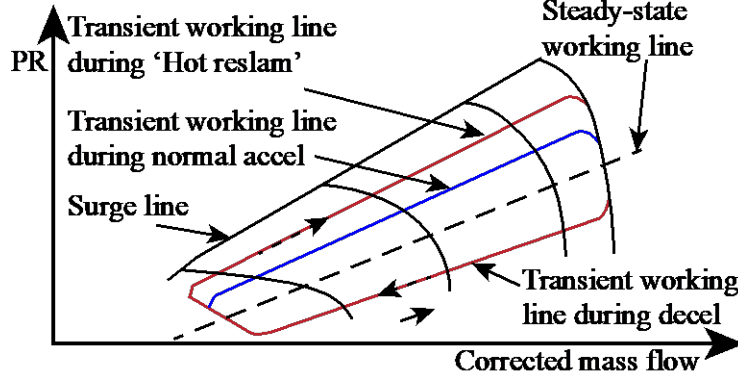
Fig. 4 Compressor transient working line under hot reslam [46].
