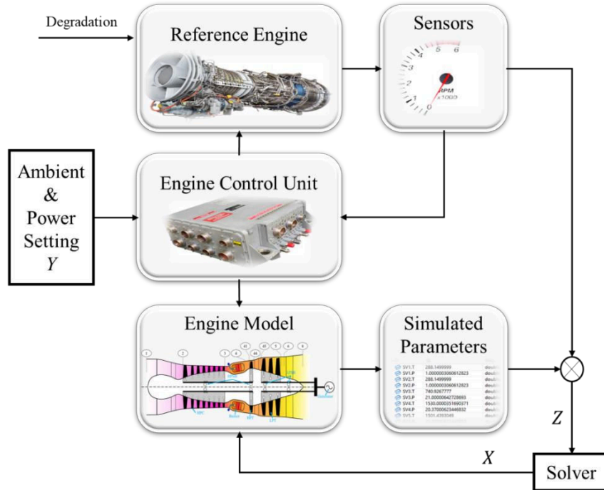
Fig. 5 Schematic of fault diagnosis [26].
