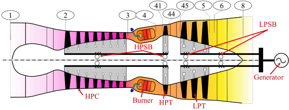
Fig. 2 Cutaway section of gas turbine in concern.
