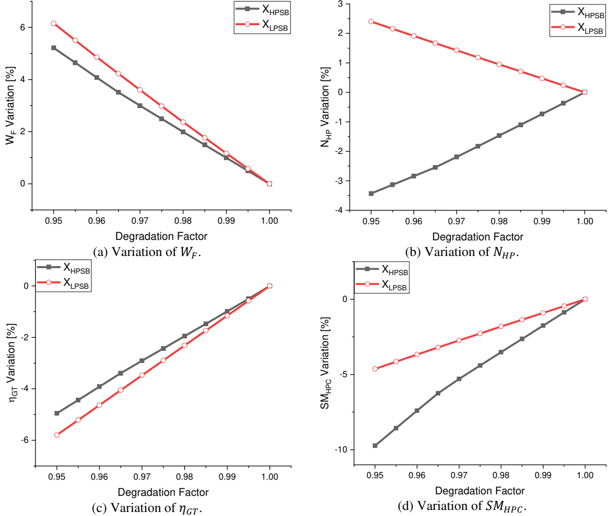
Fig. 10 Effect of shaft bearing fault on engine performance.
