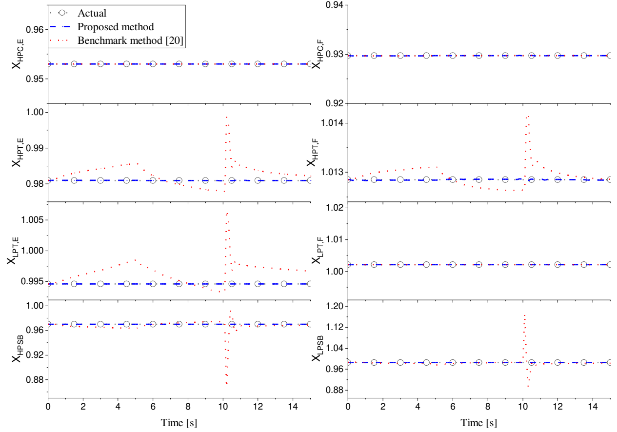
Fig. 14 Results of fault diagnosis with constant rate of degradation during a 15 s transient manoeuvre.
