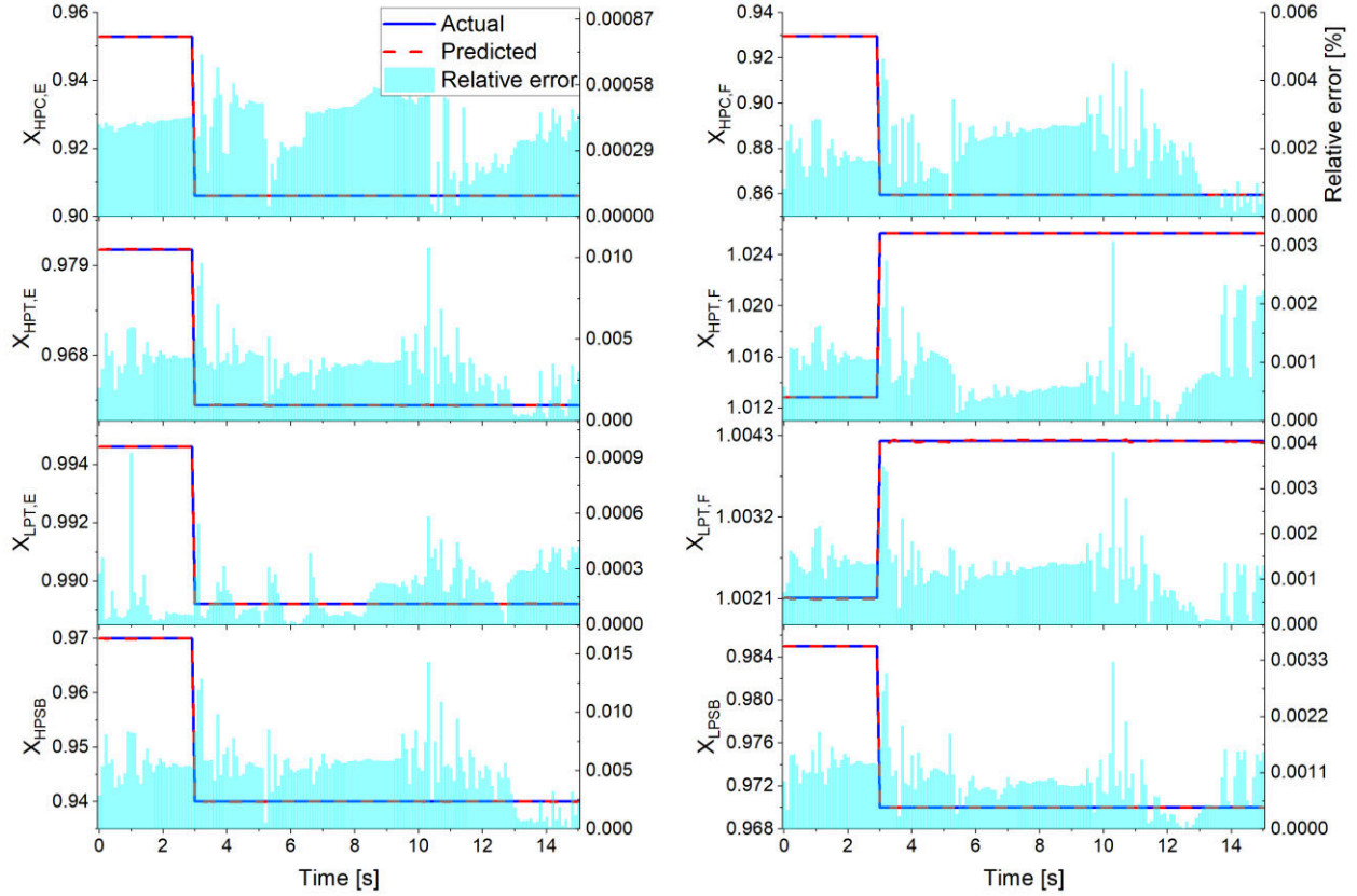
Fig. 17 Relative error of fault diagnosis with sudden failure during a 15 s transient manoeuvre.
