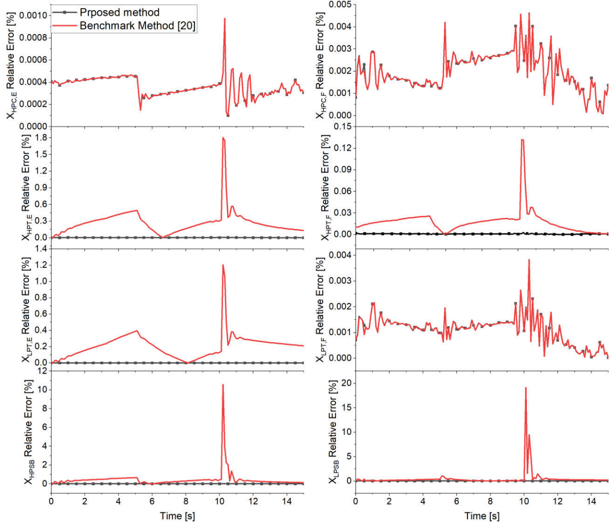
Fig. 15 Relative error of fault diagnosis with constant rate of degradation during a 15 s transient manoeuvre.
