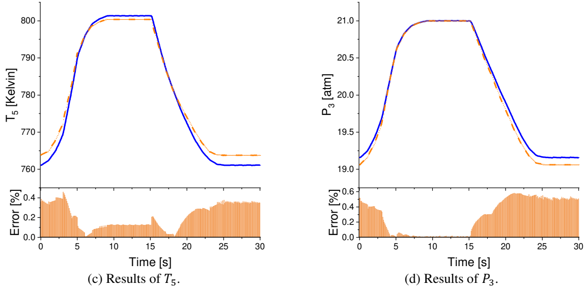
Fig. 9 Validation of model for transient manoeuvre.
