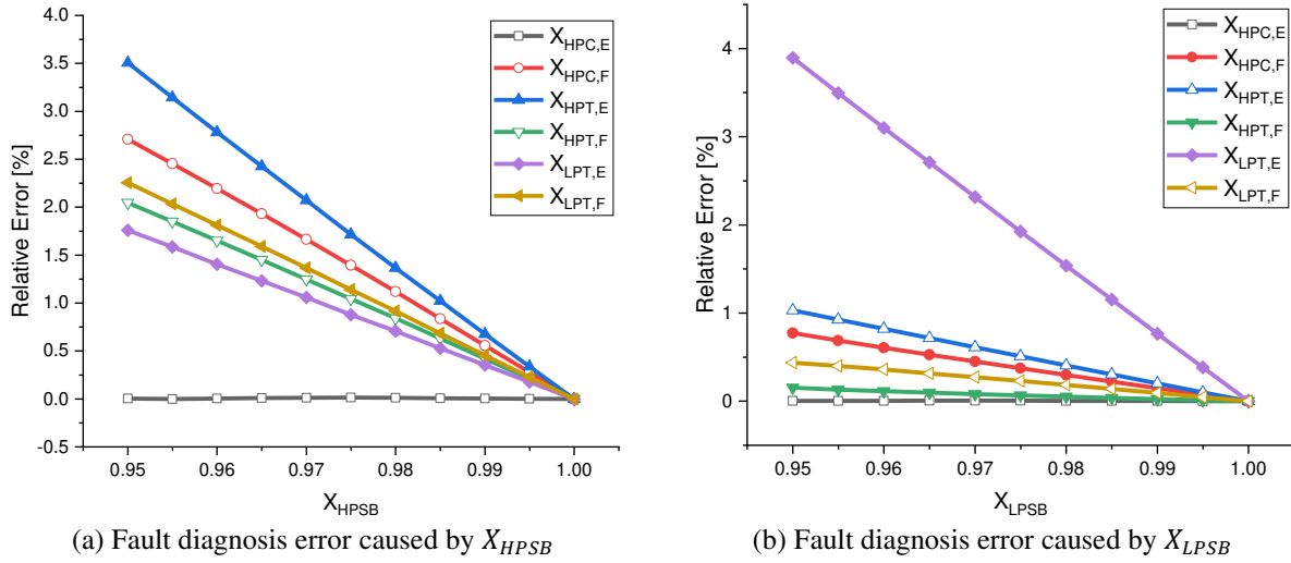
Fig. 11 Effect of shaft bearing fault on gas path analysis.
