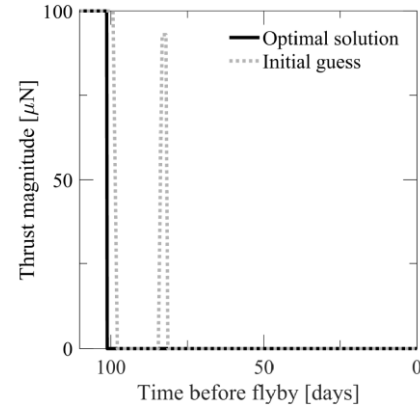
Fig. 7. Initial guess and optimal thrust history
