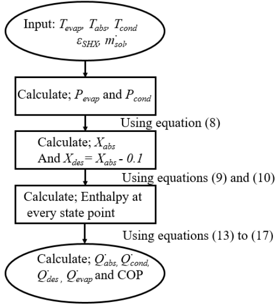
Fig. 4 Algorithm to design the VARS.
