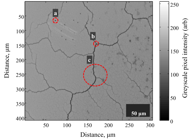
Fig. 3. Magnified image of cracked 40 nm Pd film on a glass microscope slide, taken in reflection using an optical microscope after accelerated ageing of the film (99% \text{H}_2 , 100 bar, 48 hr). Circles indicate hypothetical sensors of different active area at sites a and b (both 10.4 \mu\text{m} diameter) and c (47 \mu\text{m} diameter). Circle sizes correspond to a singlemode fibre mode field diameter and ball lens spot diameter, respectively.
