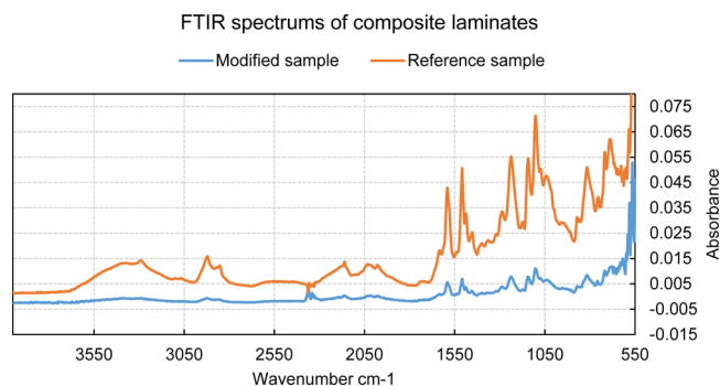
Figure 11. FTIR spectra of both modified and reference composite laminates.
