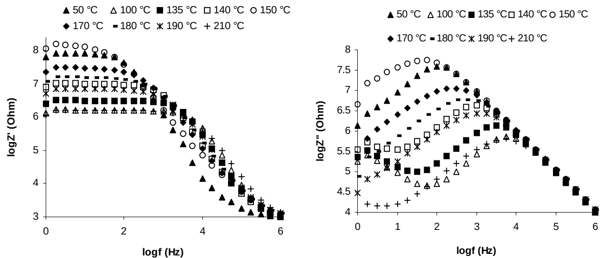
(a) Real impedance (b) Imaginary impedance Fig.6 I impedance spectrum evolution during dynamic cure at 0.25 °C/min
