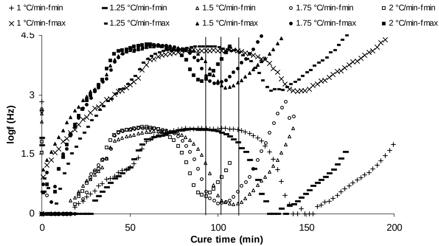
Fig.9 Frequencies of the impedance spectrum maximum and minimum in dynamic cure of RTM6 resin at high heating rates
