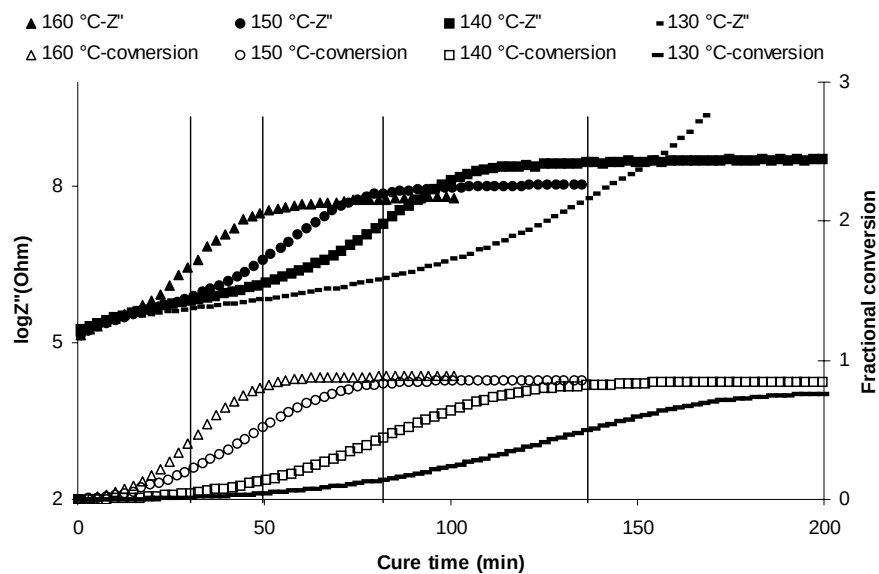
Fig.7 Imaginary impedance maximum and conversion versus time in isothermal cure
