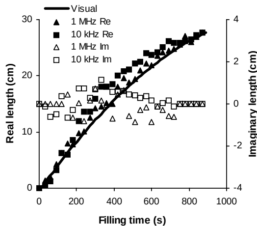
Fig. 11 Comparison of visual measurement with dielectric flow measurement for filling during resin transfer moulding of an RTM6/carbon composite
