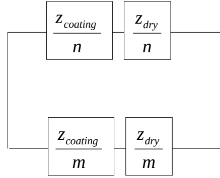
Fig. 4 Equivalent circuit representing the response of the flow sensing setup
