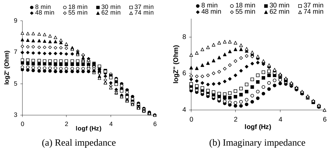
Fig.5 Impedance spectra evolution during isothermal cure at 150 °C
