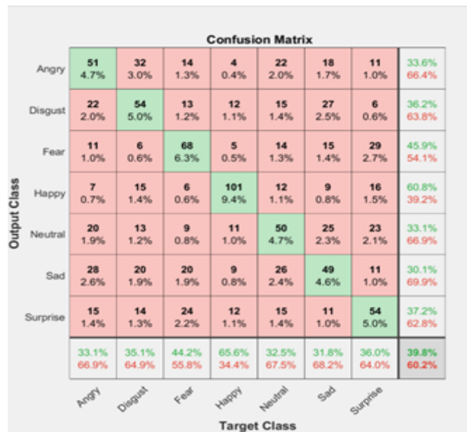
Fig. 5. Confusion Matrix shows significant result for "Happy" emotion recognition.
