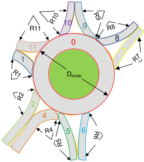
Fig. 5. Geometric parameter characteristics and entrance (#1, #4, #6, #8, #10) and exit (#2, #5, #7, #9, #11) labels of Roundabout (A) in CitySim data set
