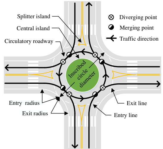
Fig. 1. Geometry elements and traffic flow characteristics at roundabouts.
