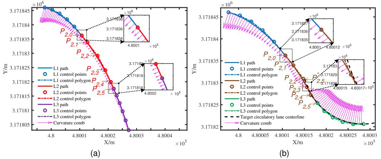
Fig. 6. The characteristics of the planned piecewise Bézier reference paths (L1, L2 and L3) in the right turn scenario (a) and entry scenario (b), including reference paths, control points, control polygons and curvature combs.
