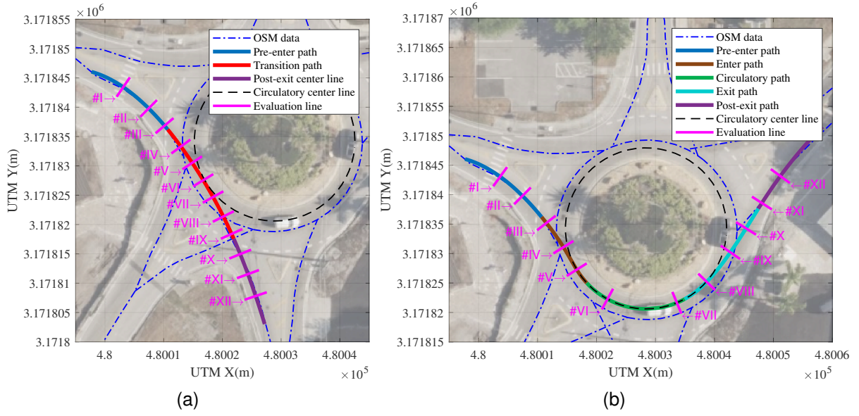
Fig. 8. The distribution of the evaluation lines on the reference paths of the Lane ID #1-#5 (a) and Lane ID #1-#7 (b) at Roundabout (A).
