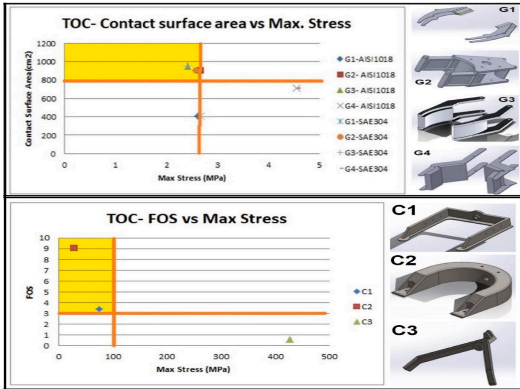
Fig. 9. ToC for (a) Gripper sub-assembly, with stress values (MPa) 2.62, 2.67, 2.41, 4.55, 2.67, 2.59, 2.4, 4.57 and surface area (cm 2 ) 407.33, 897.74, 953.2, 709.33, 407.33, 897.74, 953.2, 709.33 (b) Carrier sub-assembly, with stress values (MPa) 74.77, 28.02, 426.44 and factor of safety, 3.39, 0.59.
