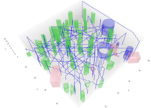
Figure 2. Generated UAS trajectories in the 3D airspace model, including linear and area flights avoiding airspace constraints.
