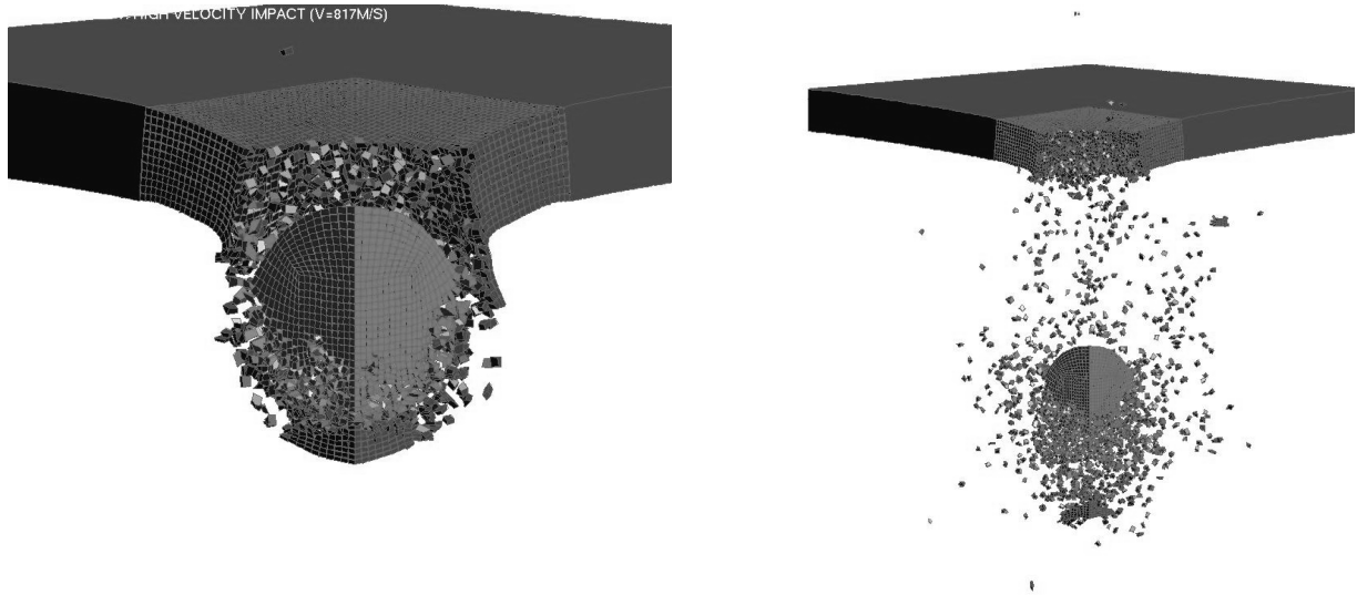
Figure 9: Target and projectile deformation at time 22 \mu\text{s} (LHS) and 50 \mu\text{s} (RHS)
