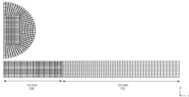
Figure 2: Discrete element model (DE: Discrete Element and FE: Finite Element)
