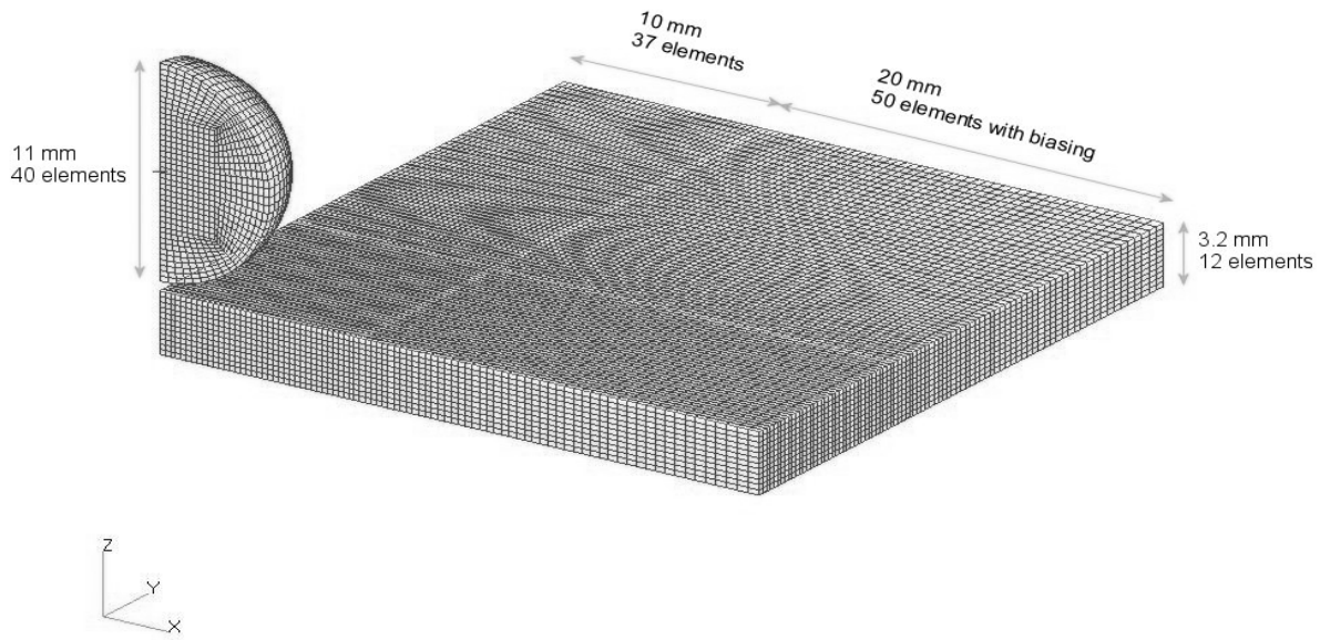
Figure 1: Finite element mesh
