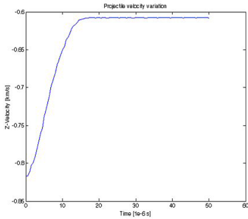
Figure 5: Projectile Z-velocity vs. time
