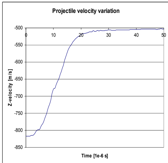
Figure 10: Projectile velocity variation
