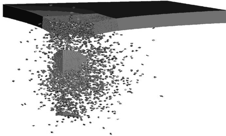
Figure 12: Configuration at time 80 \mu s, for 500 m/s case.
