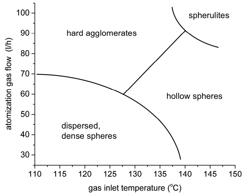
Fig. 5. A processing map for a concentration of 8.66g/100 ml and a solution feed rate of 12 ml/min shows morphology regions. 123x95mm (300 x 300 DPI)
