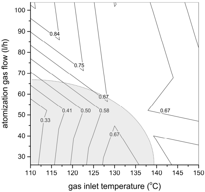
Fig. 10. A contour map of Peclet number versus gas inlet temperature and gas flow for a pump rate of 12 ml/min and feed solution concentration of 8.66 g/100 ml shows good agreement with the experimental morphology boundary (grey shaded region) for higher density, dispersed aggregates. 125x93mm (300 x 300 DPI)
