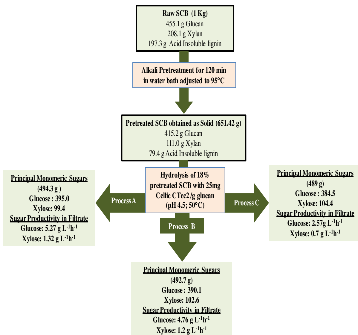
Fig. 3 Overall schematics of sugars flow during pretreatment and saccharification from one kg raw sugarcane bagasse based on the results of the present study and sugar productivities from different saccharification processes.
