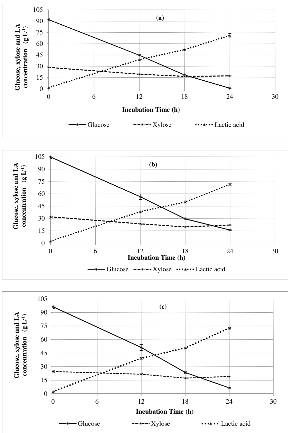
Fig. 4 Time course profile of glucose & xylose consumption and LA production by B. coagulans under pH stat conditions at 50°C and 150 rpm in filtrates obtained by (a) Process A (b) Process B (c) Process C.
