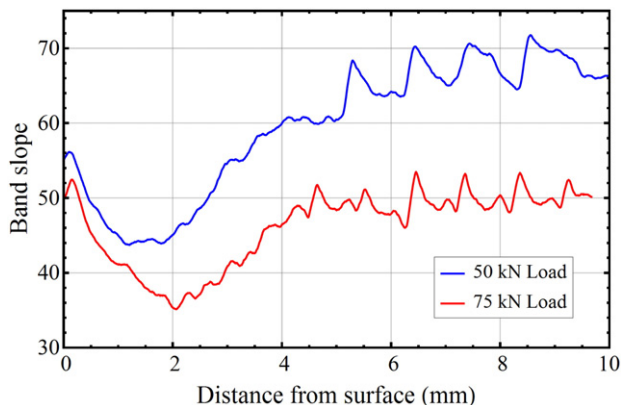
Fig. 4. EBSD pattern quality, measured by the relative band slope, for the two rolled walls plotted with vertical distance down their centre from their top surface.
