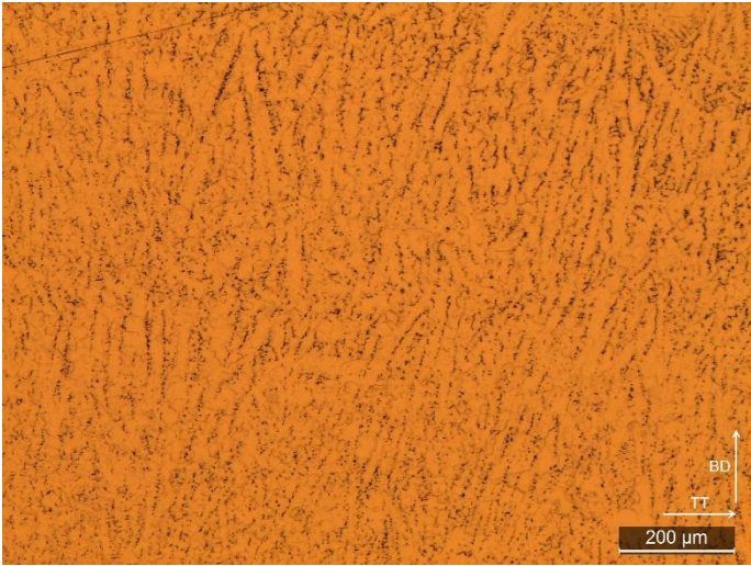
FIGURE 6: MICROGRAPH OF WORKED (W HIGH) SHOWING DISTURPTED DENDRITIC STRUCTURE.
