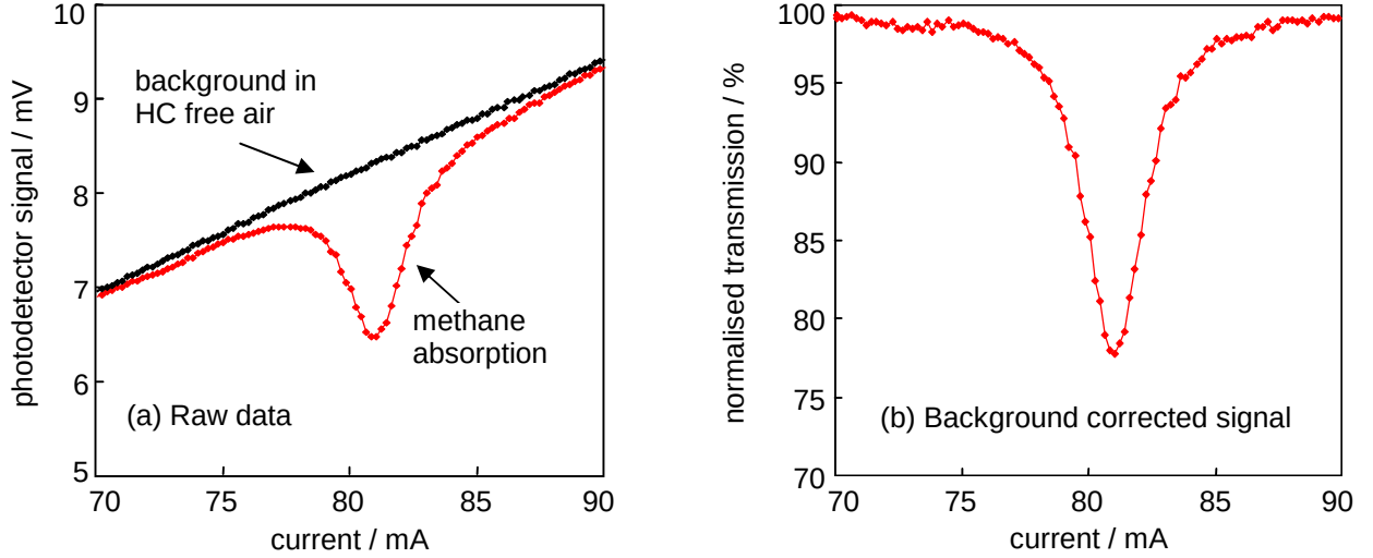
Figure 6. Examples of detected signals recorded while the laser wavelength was scanned across a single methane line at 1651nm. (a) Raw data from the detector for HC free air and for a methane concentration of 5770 ppm. (b) Methane transmission normalized by division by the background signal.
