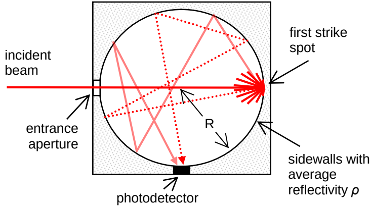
Figure 1. Simplified model of an integrating sphere, showing the incident beam making a first pass across the cell to the first strike spot. Two examples are shown of light beams making subsequent random multiple passes across the cell.
