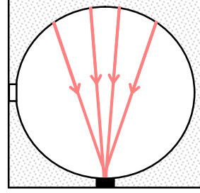
(c) Final pass for detector with restricted field of view: mean pathlength 1.85 R
