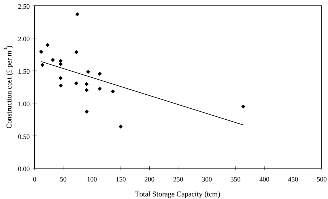
Figure 6-13. Reported construction costs (£ per m³ gross storage capacity) for lined reservoirs.
