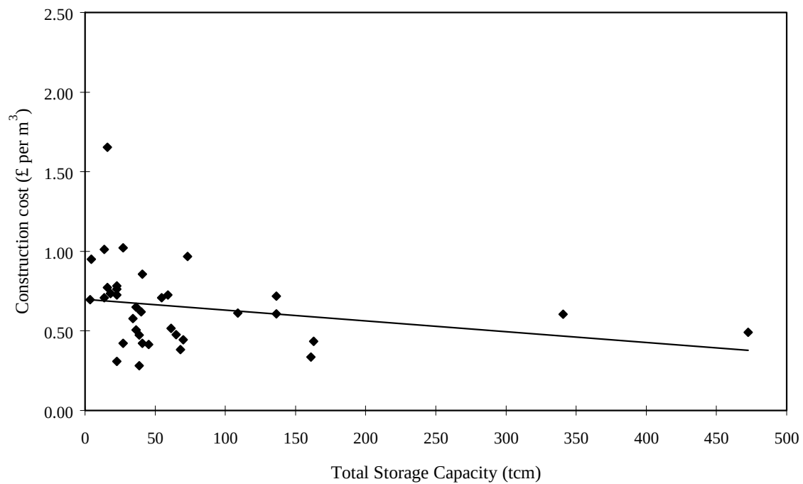
Figure 6-12. Reported construction costs (£ per m³ gross storage capacity) for unlined reservoirs.
