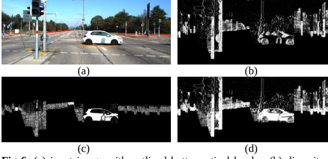
Fig 6. (a) input image with outlined bottom stixel border, (b) disparity membership m_d(u, v) ; (c) colour membership m_c(u, v) ; (d) joined membership m(u, v) (best seen in color)
